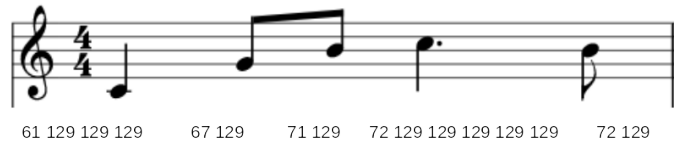
Figure 2: Integer representation of a monophonic melody. Values 0–127 represent MIDI “note on”, 128–“note off”, and 129–“no change”. The first quarter note is represented by four integers where the first denotes the MIDI pitch and the next three indicate that there is no change for the next three semi-quavers.
