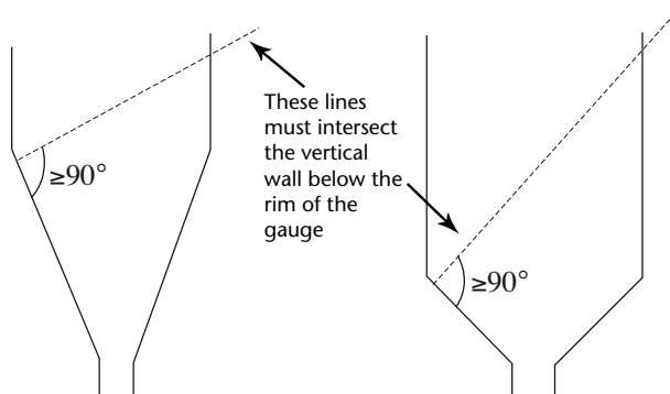
Figure 6.2. Suitable collectors for rain gauges
