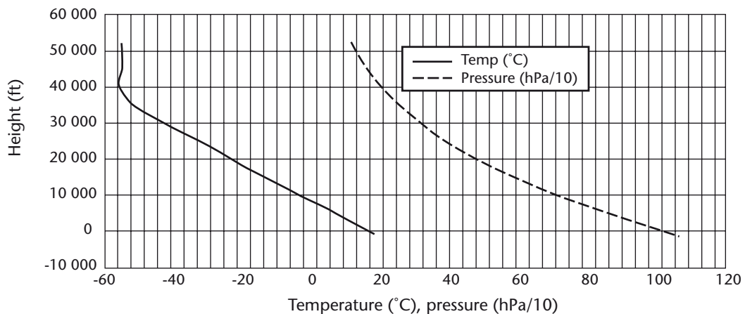
Figure 3.3. ICAO Standard Atmosphere
