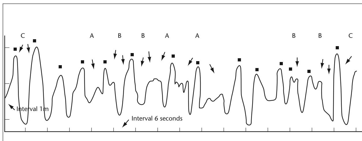
Figure 4.1. Typical sea and swell waves as shown by a wave-height recorder
