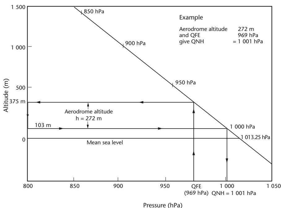
Figure 2.1. The relation between QFE and QNH
