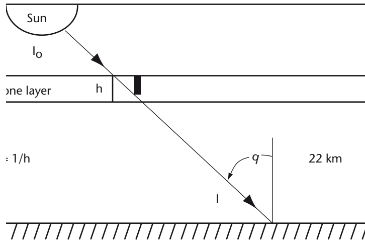
Total ozone by spectrophotometer
