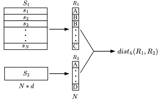
Figure 5: The process of transmitting S to representation R and computing the Hamming Distance
