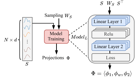
Figure 3: Learning projections in DARKER
