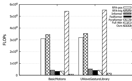
Figure 10: FLOPs of all methods on two datasets
