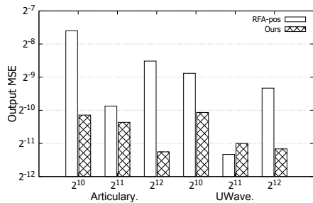
Figure 15: Approximation error to softmax attention
