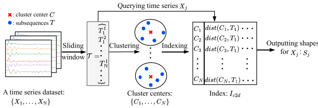
Figure 8: Extracting a shape for input X_j in cluster C_i
