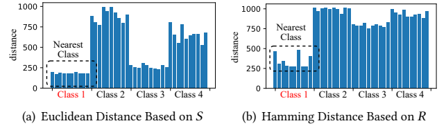
Figure 6: The distance of a selected instance from Class 1 to others
