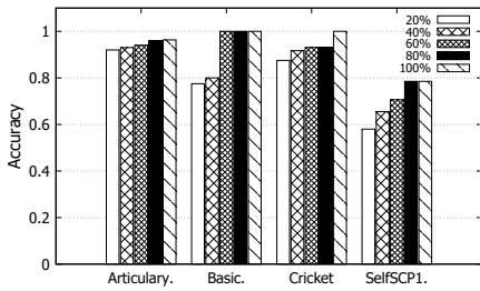
Figure 12: Accuracy on ratios for learning projections.
