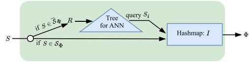
Figure 7: PINDEX of searching \Phi for S
