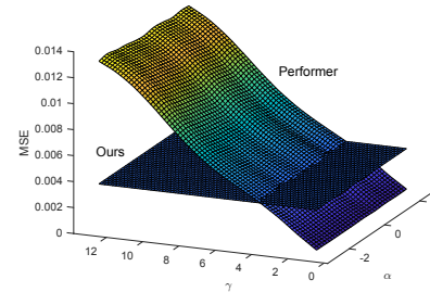
Figure 1: The approximation error of softmax in Performer [5] and our method. Two matrices, Q and K , are initialized consisting of N pairs of query and key vectors. Then, the key vector is scaled with a scalar \gamma and rotated with an angle \alpha .
