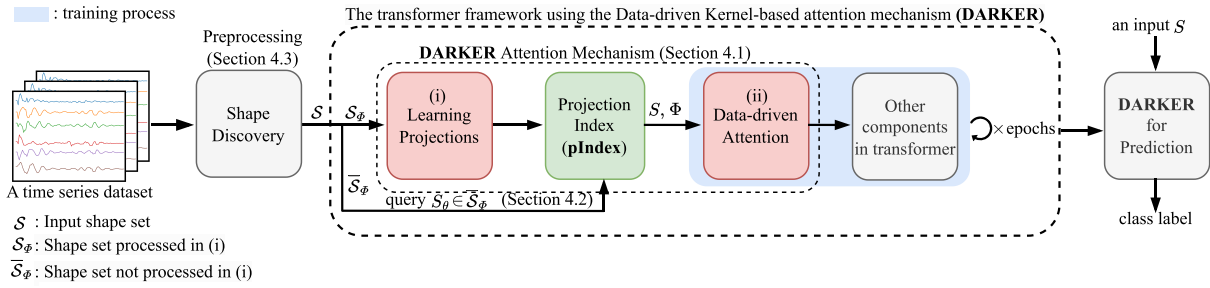
Figure 2: The overview of DARKER
