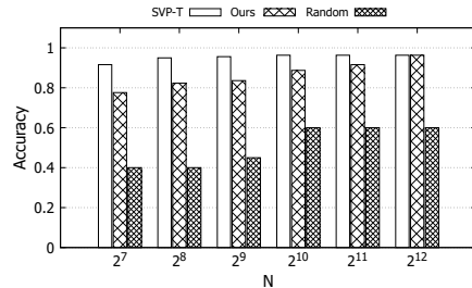
Figure 14: Accuracy on three shape discovery methods
