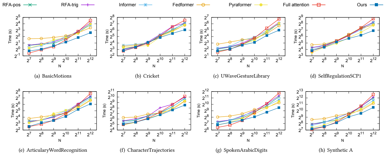
Figure 9: Training time on varying the number of shapes N
