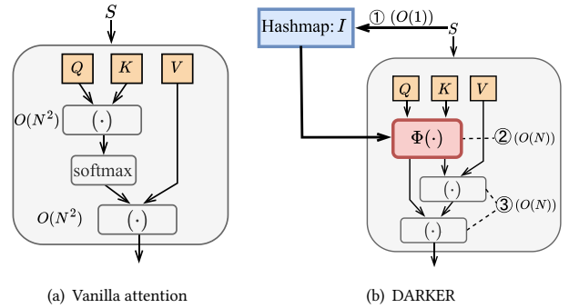
Figure 4: Vanilla and DARKER attention mechanism
