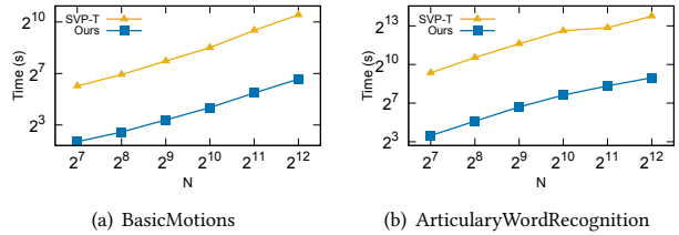
Figure 13: Efficiency on shape discovery of SVP-T, and ours
