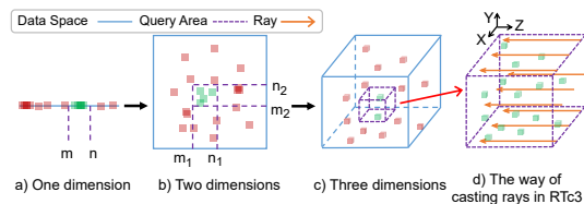
Figure 3: Data distribution in multi-dimensional spaces
