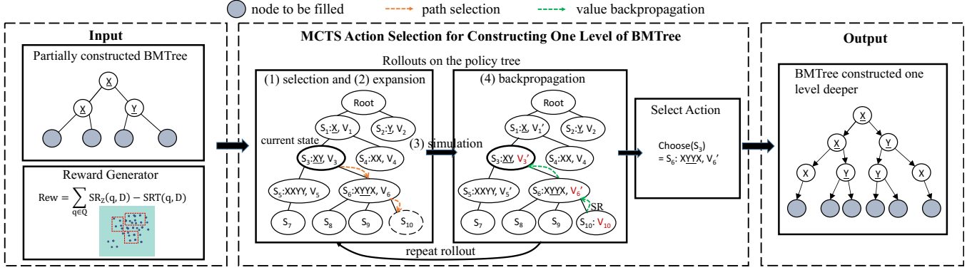
Figure 5: Workflow of Monte Carlo Tree Search Based BMTree construction.
