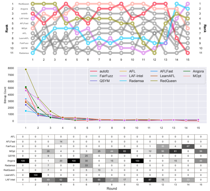
(b) Evaluation of autofz decision on exiv2
