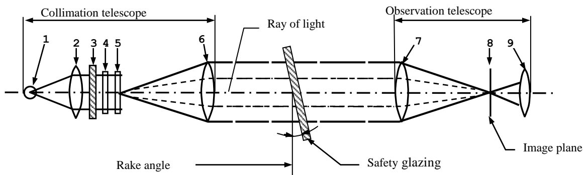
Figure 13 Apparatus for collimation-telescope test
