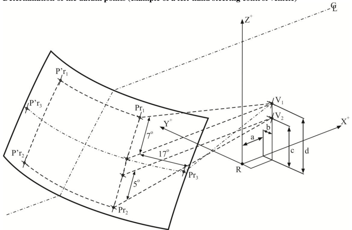
Figure 3 Determination of the datum points (example of a left-hand steering control vehicle)
