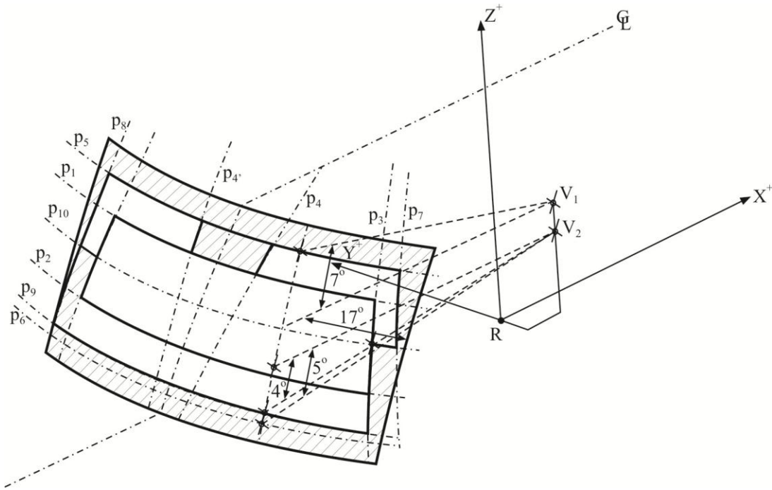
Figure 2b Reduced test area "B" (example of a left-hand steering control vehicle) - upper obscuration area as defined in paragraph 2.4.2.1.
