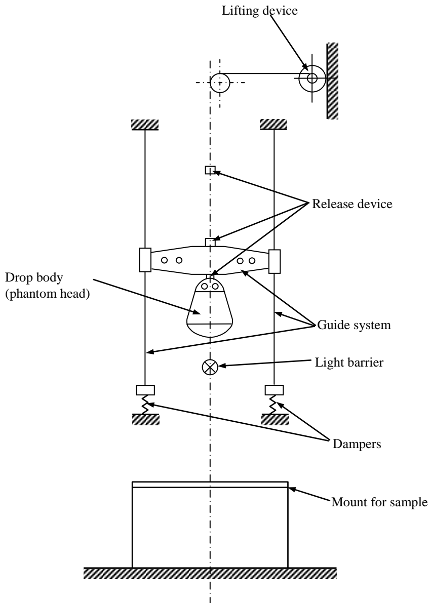
Test apparatus for the headform experiment with deceleration measurement
