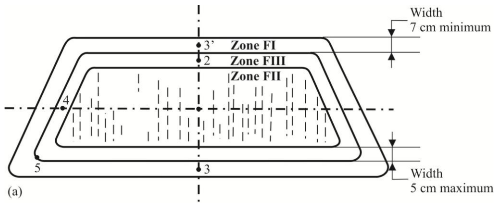
Figure 2 Prescribed points of impact for windscreens
