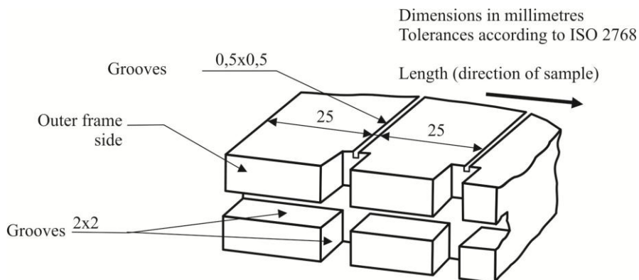
Figure 19 Example of section of lower U-frame design for wire support facility
