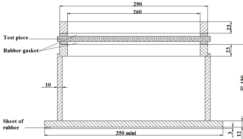
Figure 1 Support for ball tests
