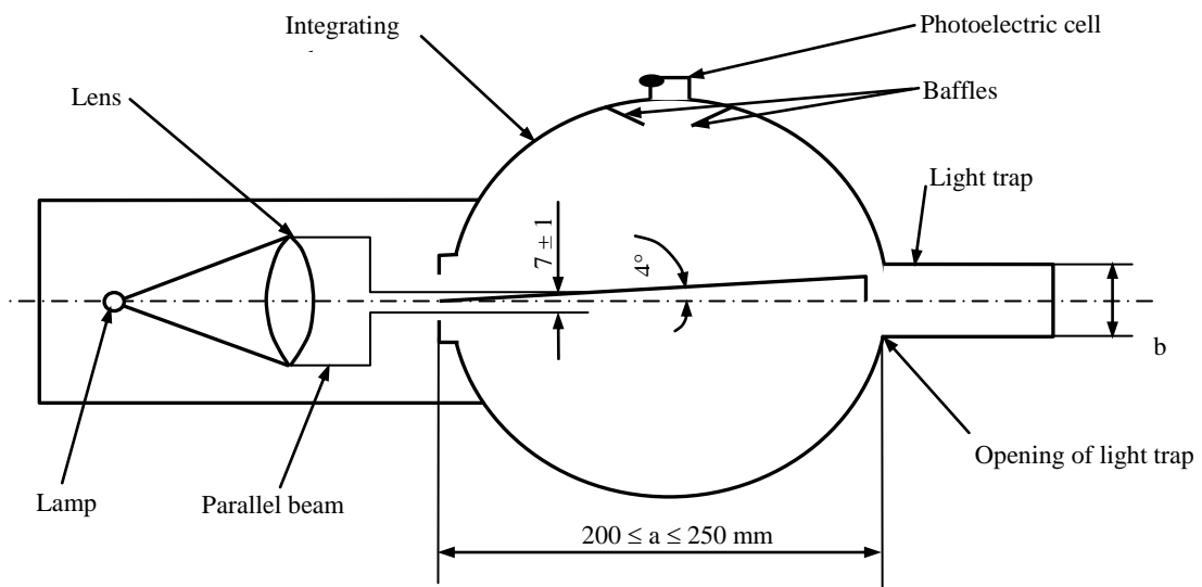
Figure 5 Hazemeter
