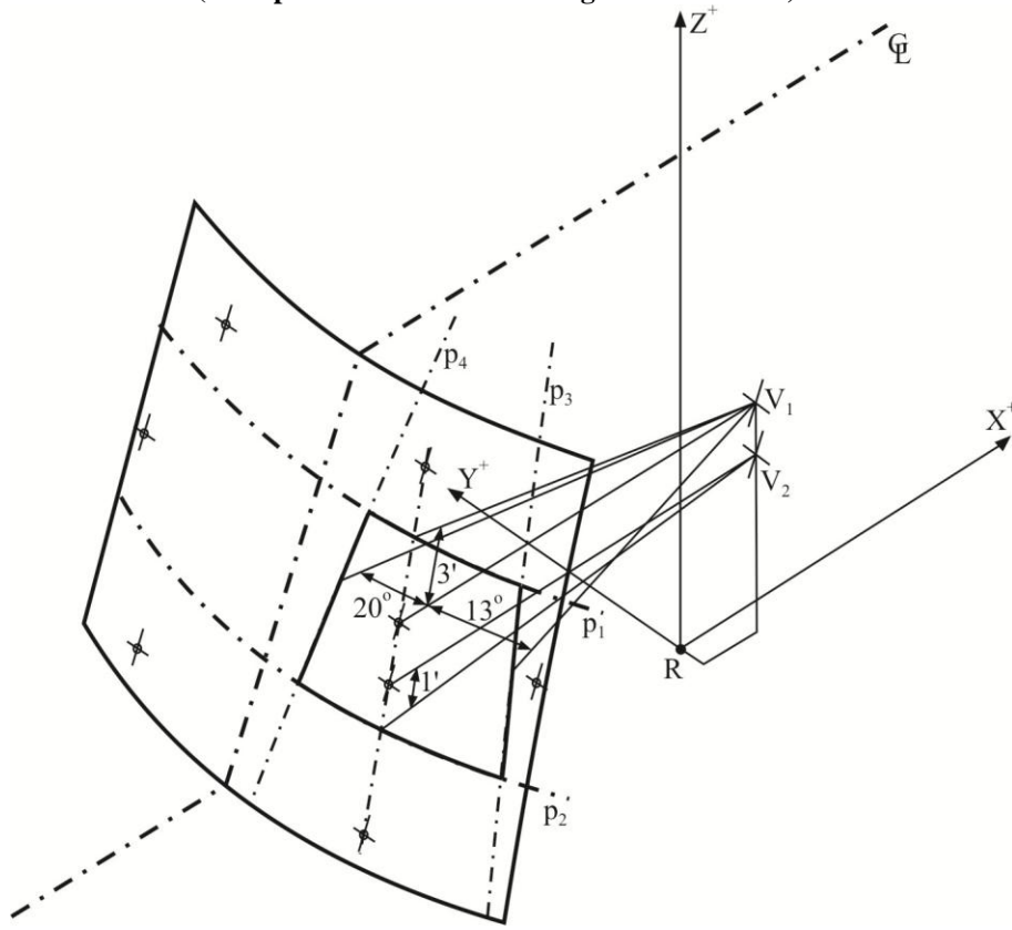
Figure 1a Test area "A" (example of a left-hand steering control vehicle)
