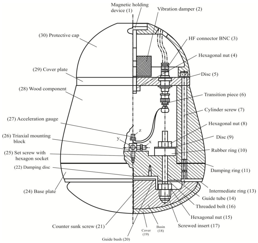
Figure 2.1 10 kg Headform
