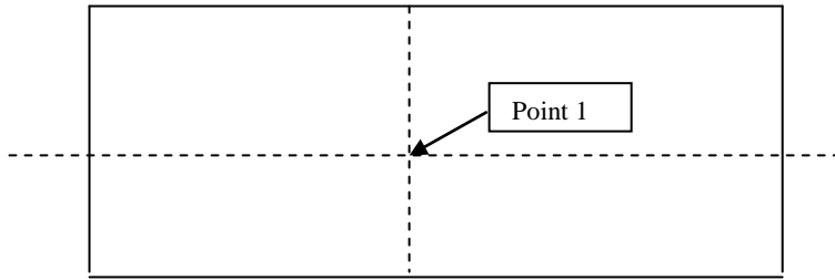
Figure 3 Prescribed points of impact for uniformly toughened glass panes
