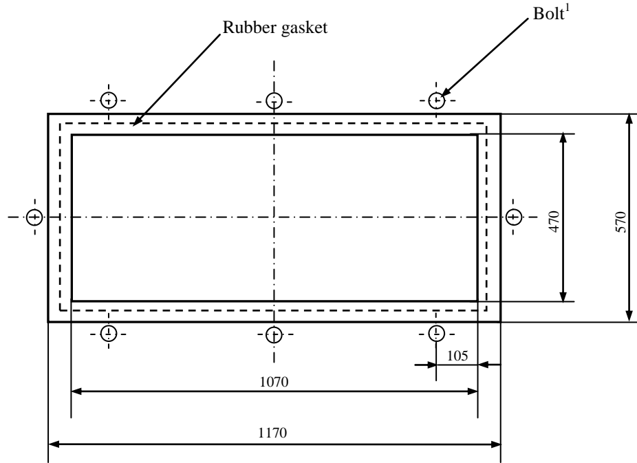
Figure 3 Support for headform tests
