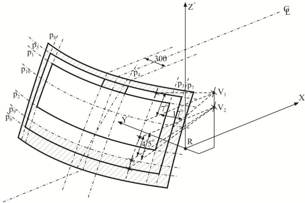
Figure 2a Reduced test area "B" (example of a left-hand steering control vehicle) - upper obscuration area as defined in paragraph 2.4.2.2.
