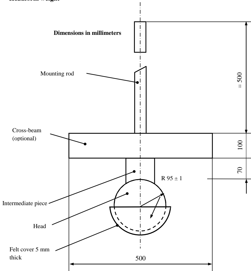
Figure 2 Headform weight
