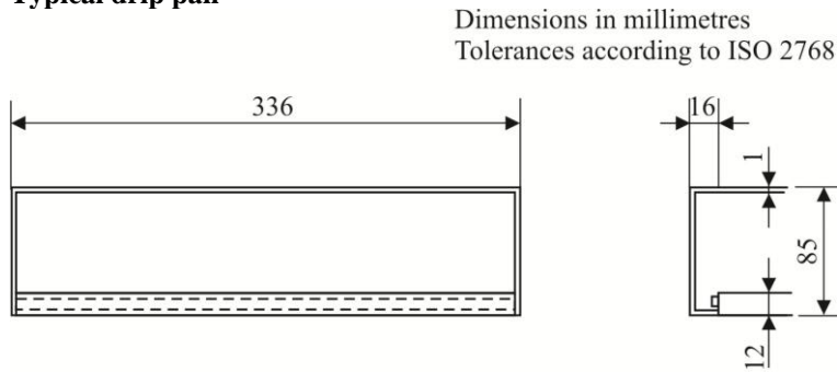
Figure 18 Example of sample holder
