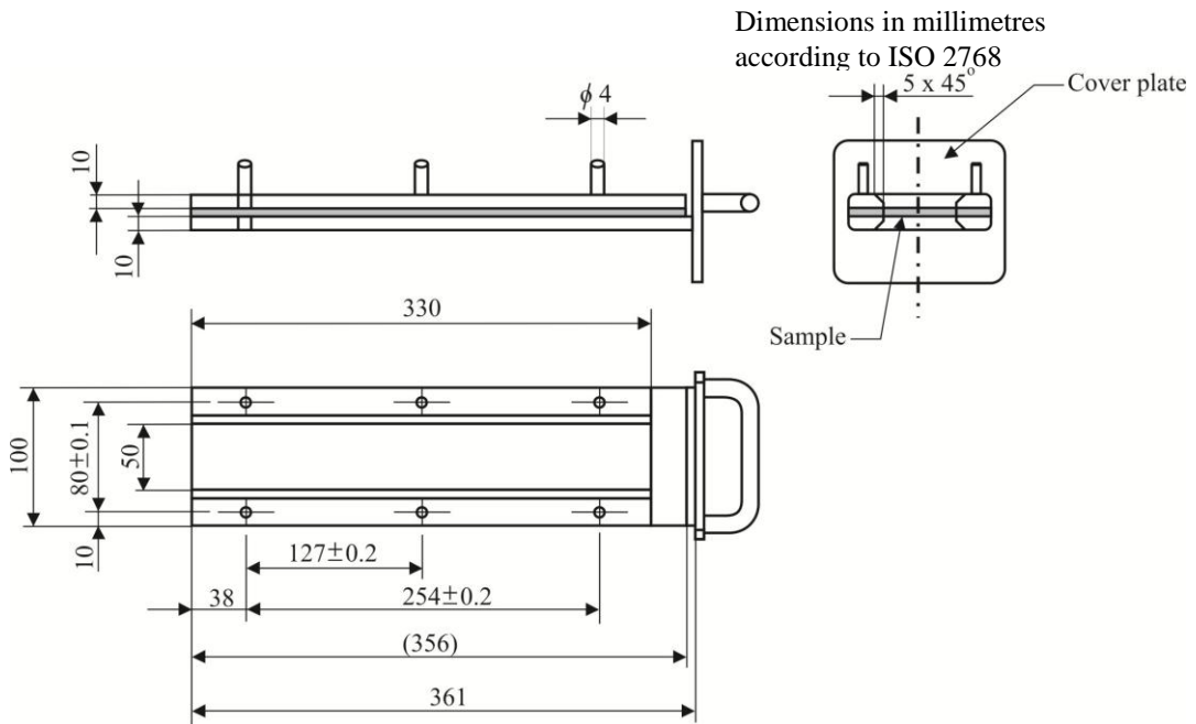
Figure 19 Example of section of lower U-frame design for wire support facility
