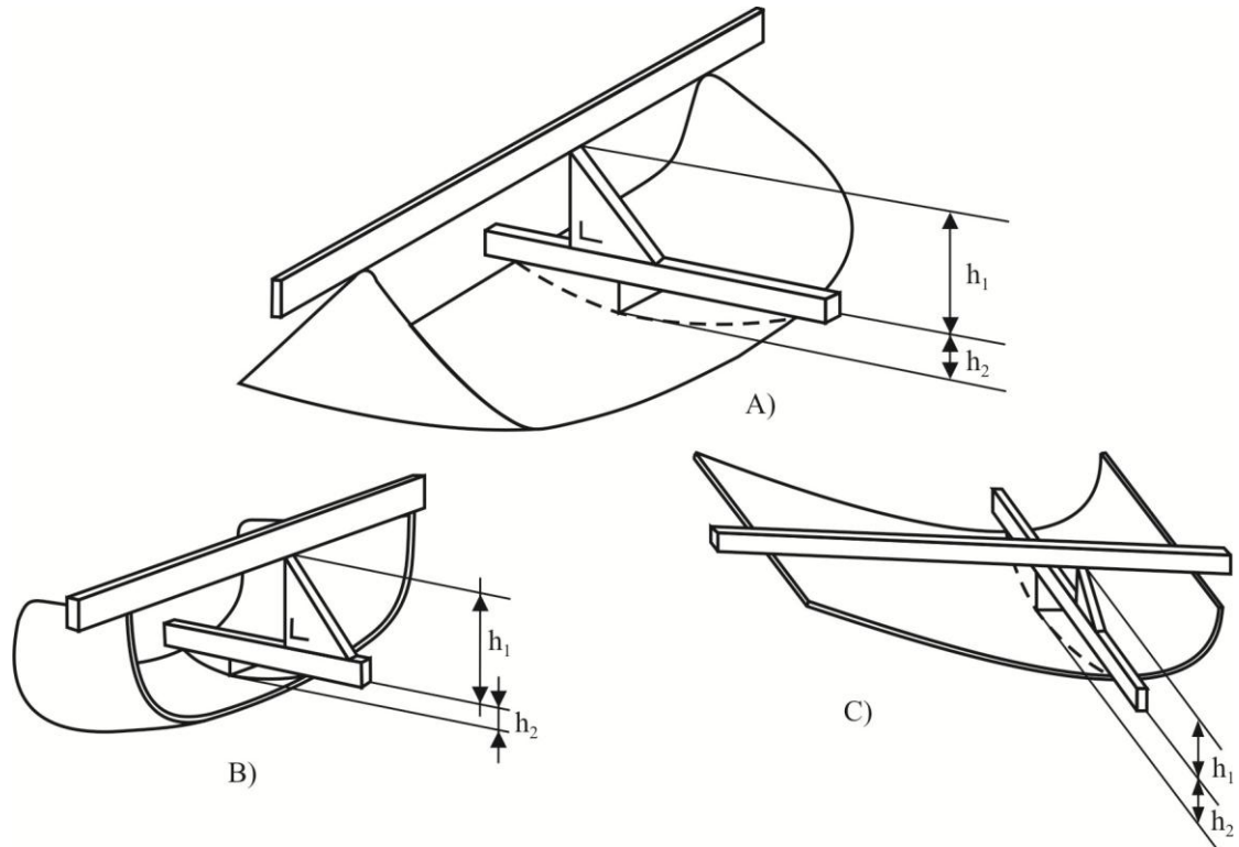
Figure 1 Determination of the height of segment 'h'
