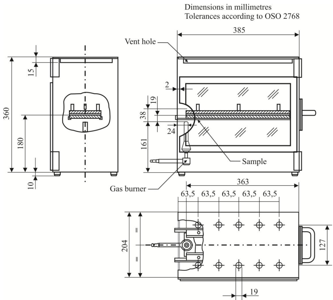
Figure 16 Example of combustion chamber
