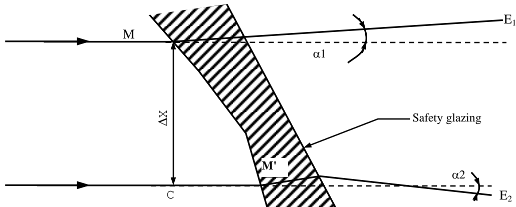
Figure 6 Diagrammatic representation of optical distortion
