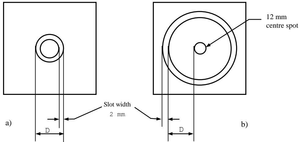
Figure 12 Arrangement of apparatus
