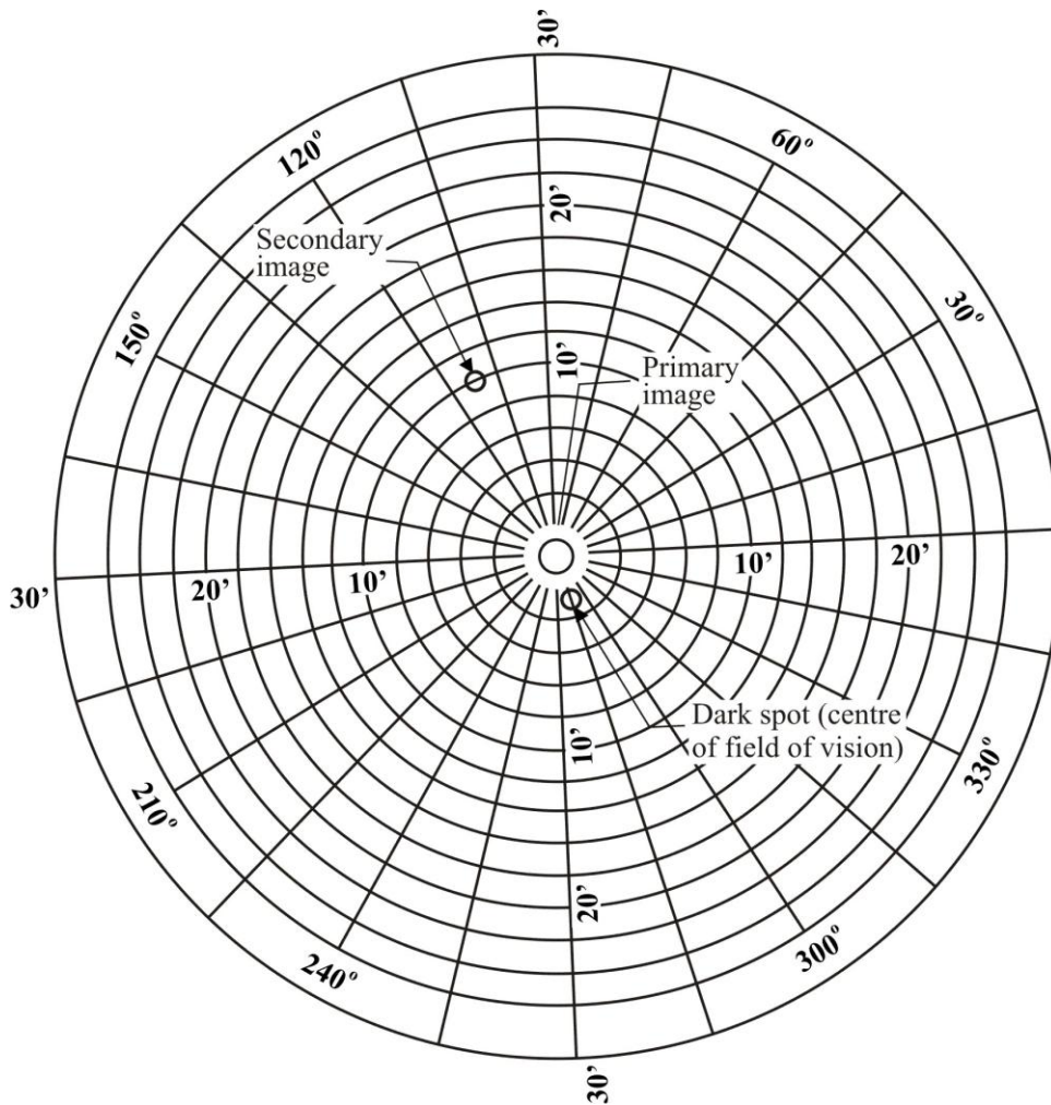
Figure 14 Example of observation by the collimation-telescope test method
