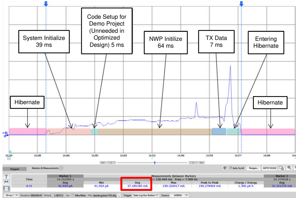
Figure 2-31. Transceiver Mode Close-Up View
