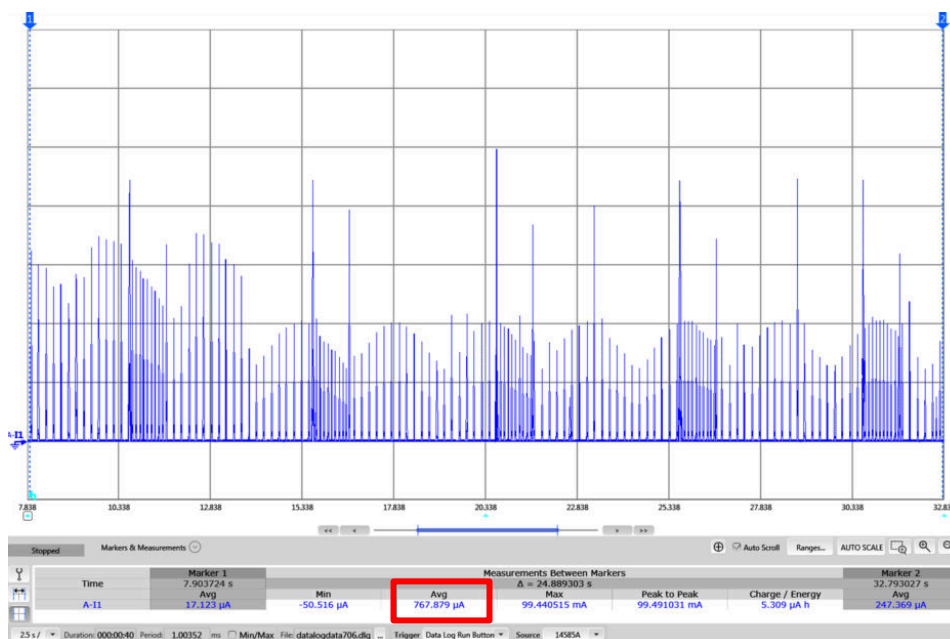
Figure 2-36. CC3235SF Device in Always Connected Mode (UDP)
