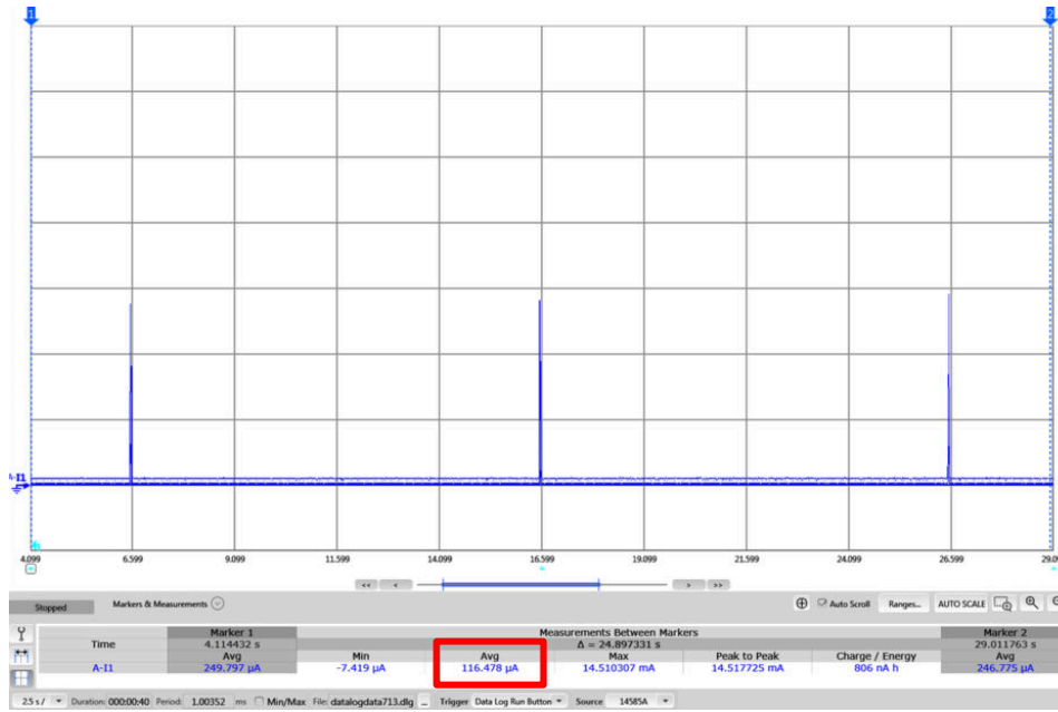
Figure 2-27. CC3135 Device in LPDS Mode
