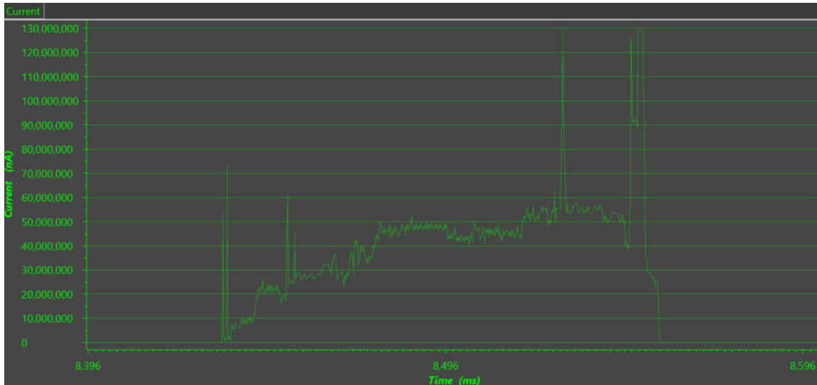
Figure 2-24. Average Current Measurement With EnergyTrace™
