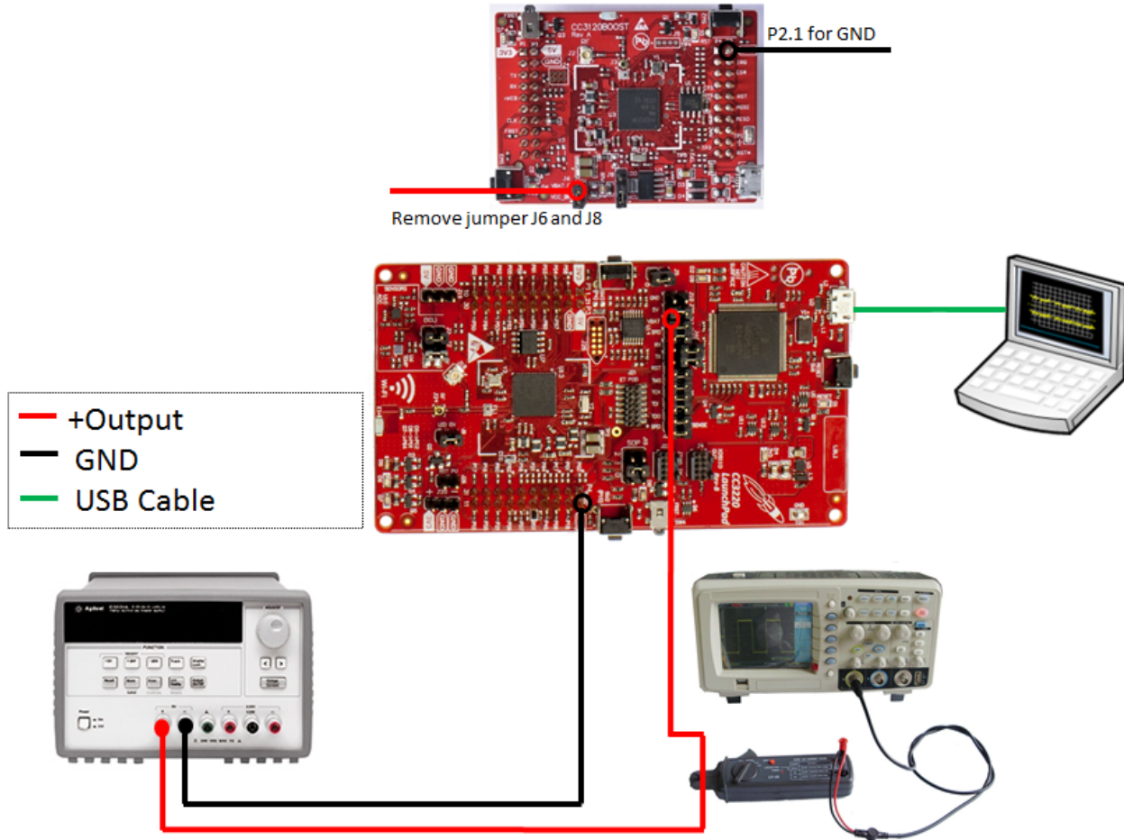
Figure 2-13. Oscilloscope With Current Probe Test Setup
