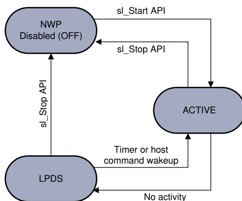
Figure 1-2. Transitions Between States
