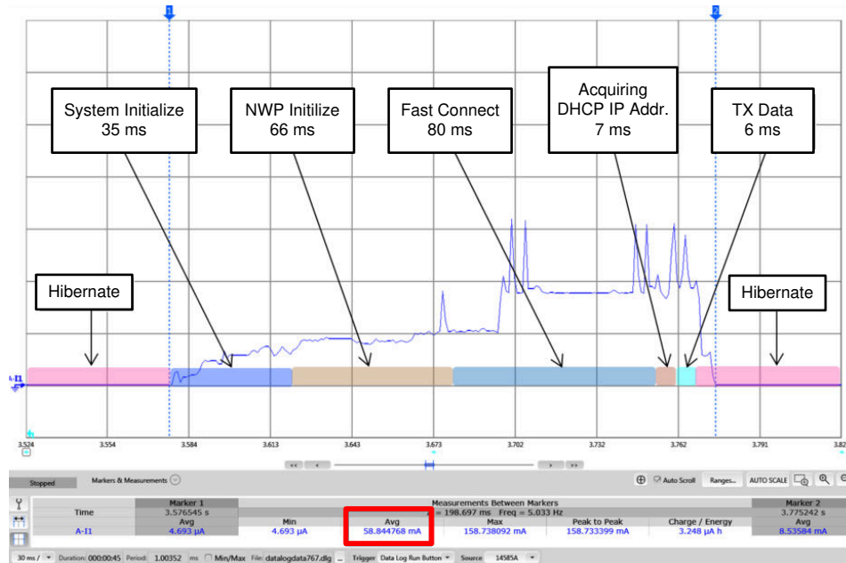
Figure 2-34. Intermittently Connected Mode Close-Up View
