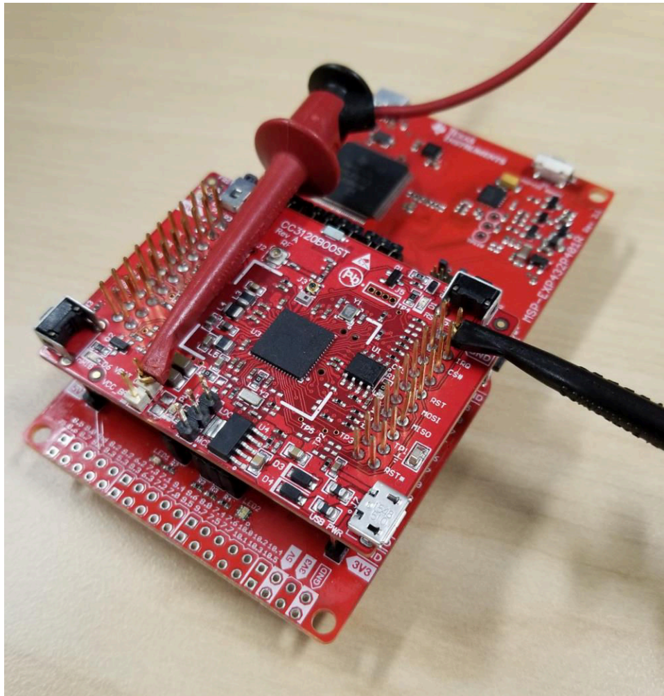
Figure 2-5. DC Power Analyzer Connection to CC3135 Device
