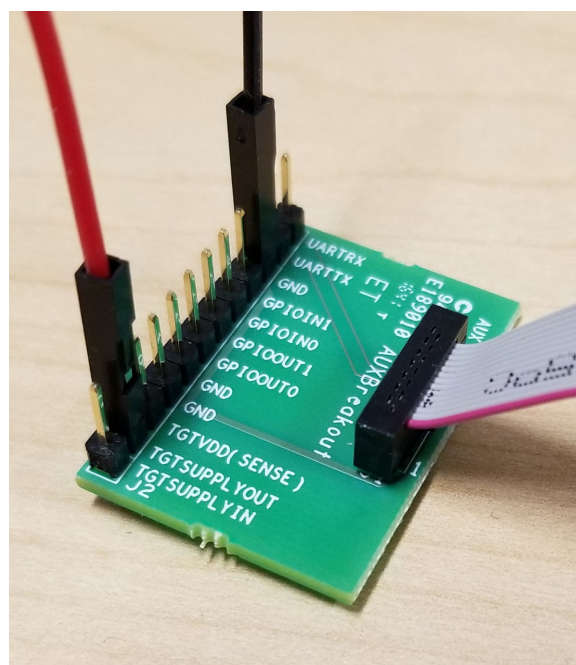
Figure 2-18. Breakout Board Connection
