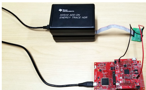
Figure 2-22. CC3135 Device Test Setup With XDS110 System
