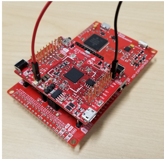
Figure 2-17. XDS110 ETHDR Connection to CC3135 Device
