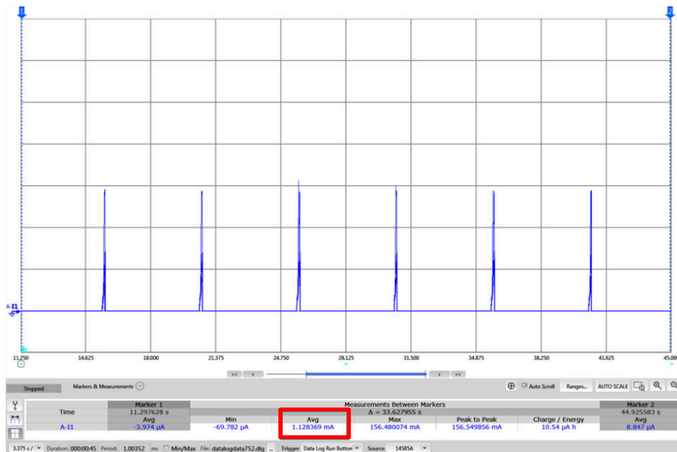
Figure 2-32. CC3135 Device Intermittently Connected Mode
