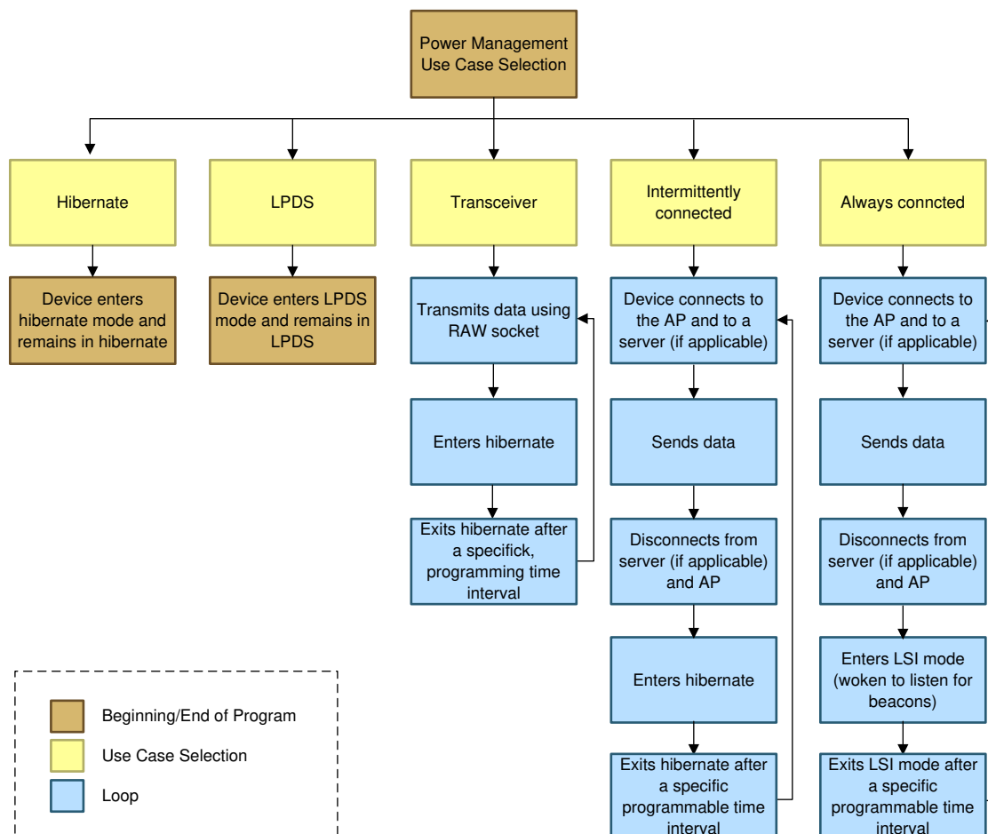
Figure 2-4. Power Management Use-Case Selection Flowchart
