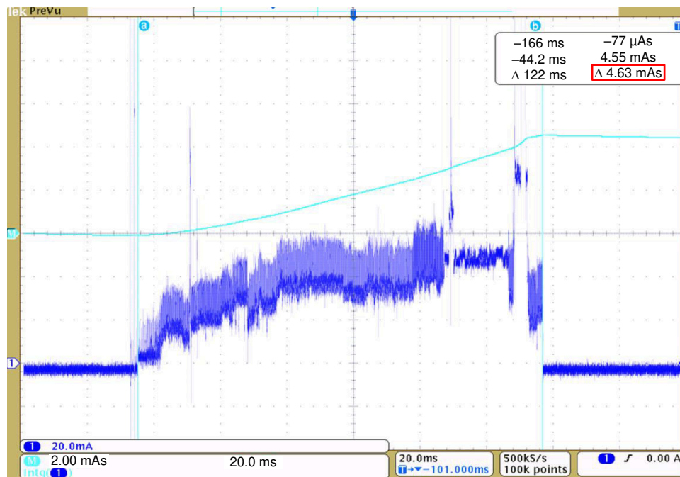
Figure 2-14. Current Measurement With Current Probe
