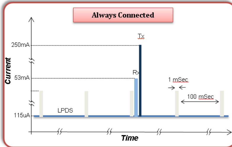
Figure 1-4. Always Connected Test Case
