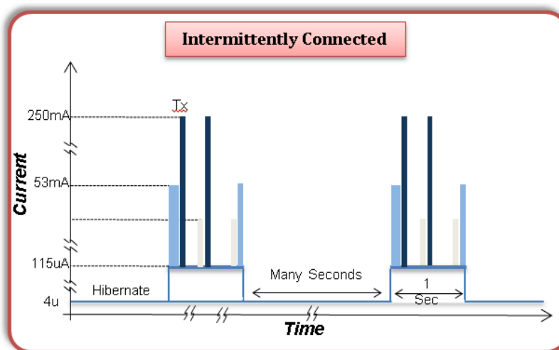
Figure 1-3. Intermittently Connected Test Case
