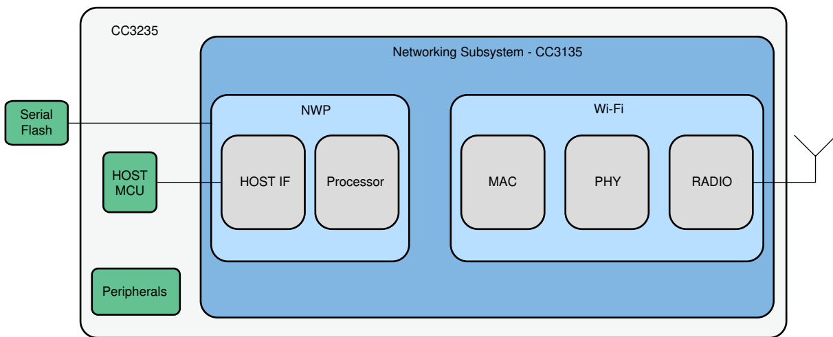
Figure 1-1. CC313x and CC323x Device Block Diagram
