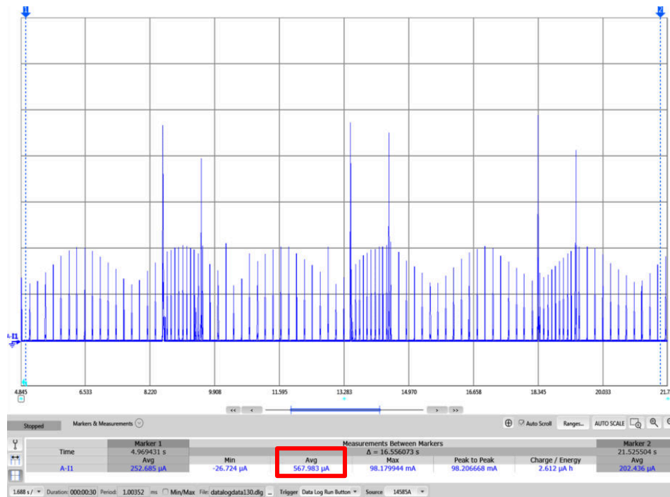
Figure 2-35. CC3135 Device in Always Connected Mode (UDP)
