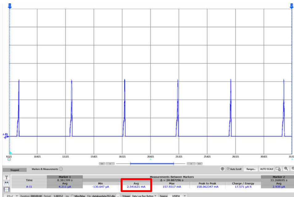
Figure 2-33. CC3235SF Device in Intermittently Connected Mode
