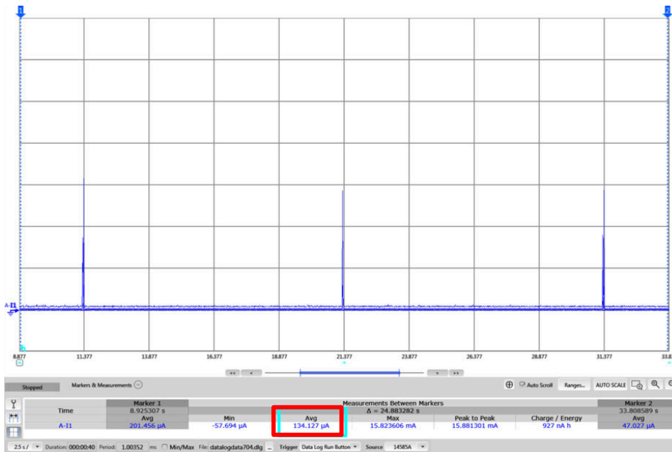
Figure 2-28. CC3235SF Device in LPDS Mode
