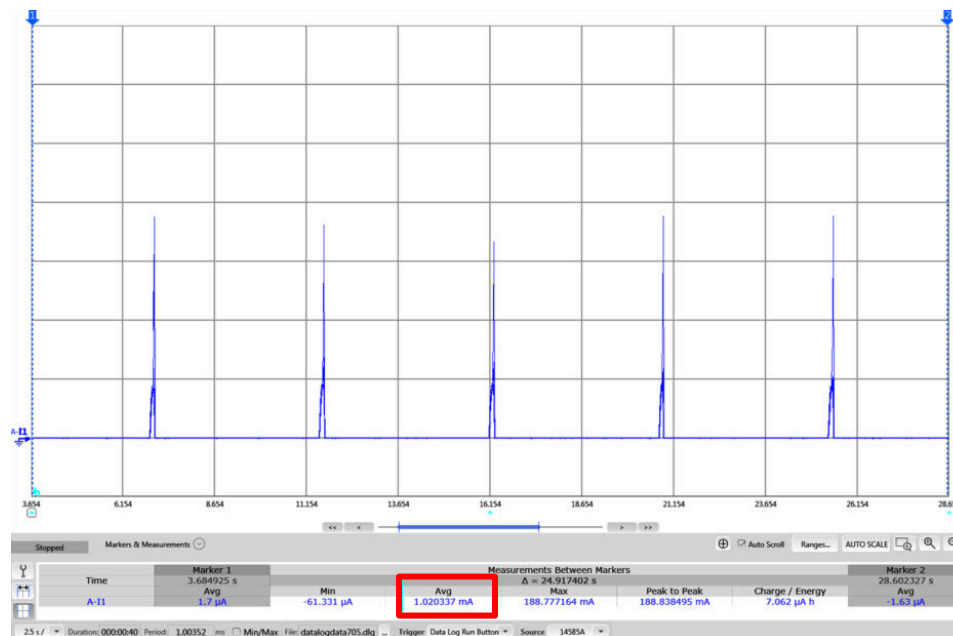
Figure 2-30. CC3235SF Device in Transceiver Mode
