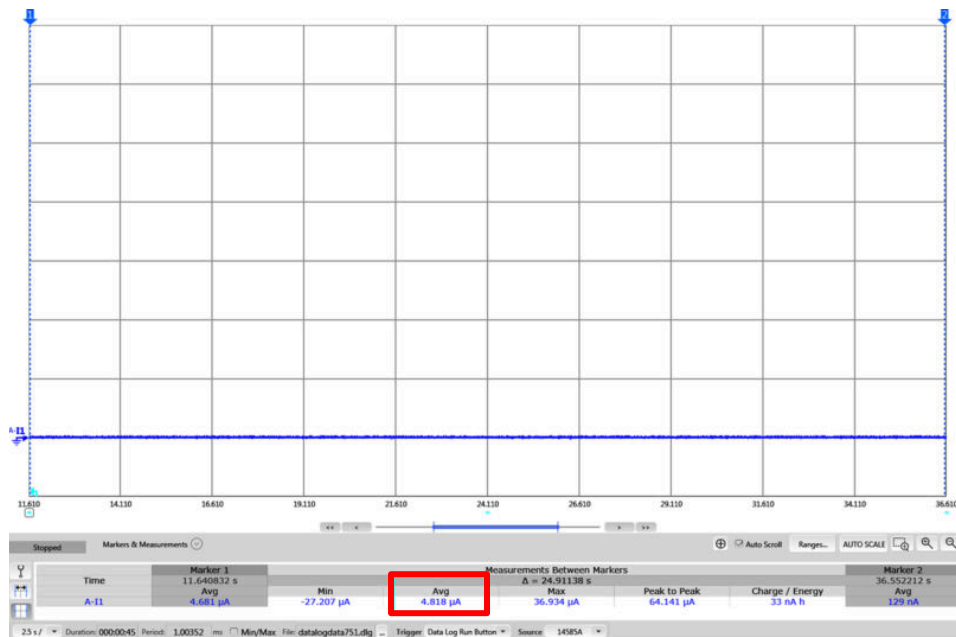
Figure 2-25. CC3135 Device in Hibernate Mode
