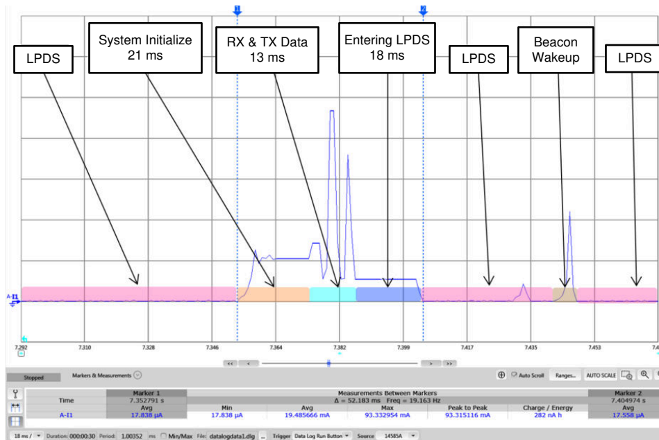
Figure 2-37. Always Connected Close-Up View
