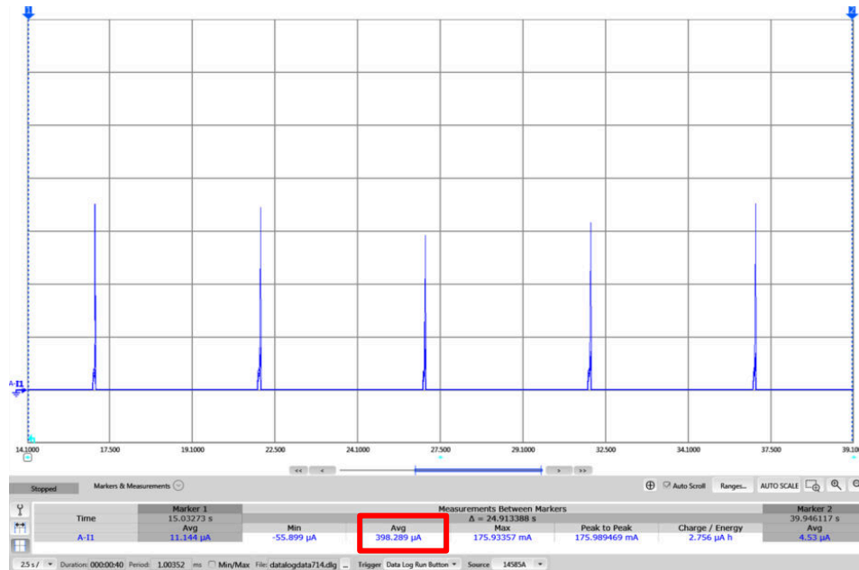
Figure 2-29. CC3135 Device in Transceiver Mode
