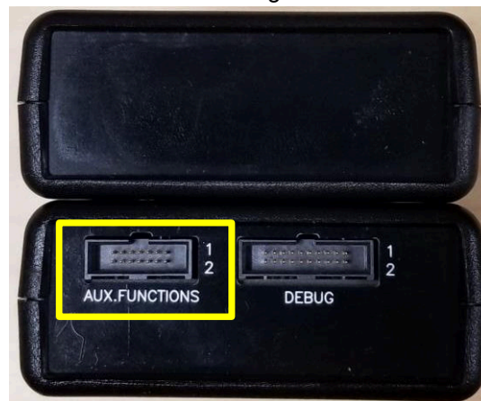
Figure 2-20. XDS110 Auxiliary Interface
