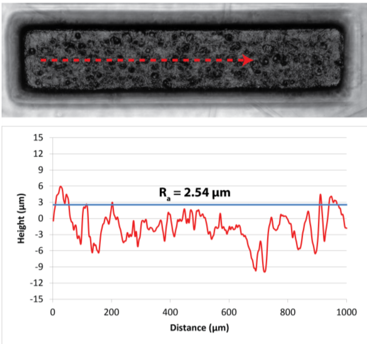
Fig. S1. (a) A representative micrograph of a bottom-facing trench and the orientation of line-scans measured using a stylus profilometer. (b) A representative line-scan of median roughness ( R_a = 2.54 \mu\text{m} ).
