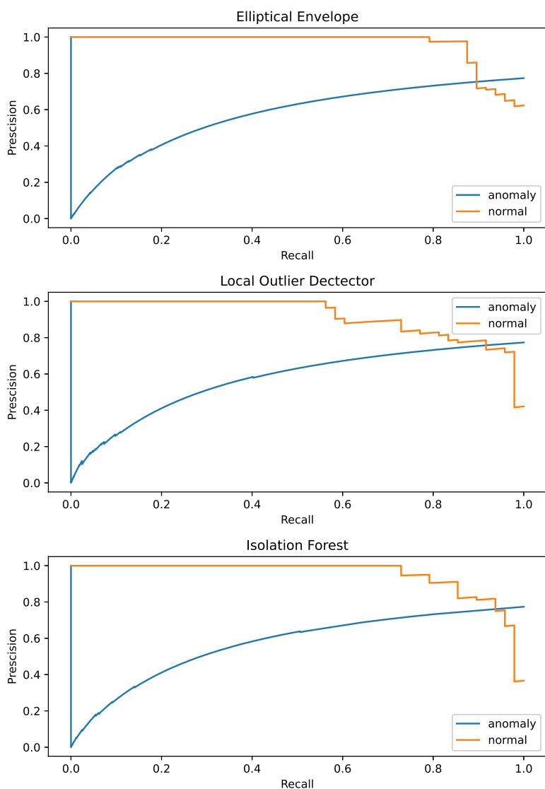
FIG. 1. Precision-Recall curves for anomaly detection models.
