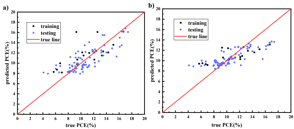
Figure S4 The plots of the relationship between the true PCE and the predicted PCE predicted by (a) KNN and (b) SVM
