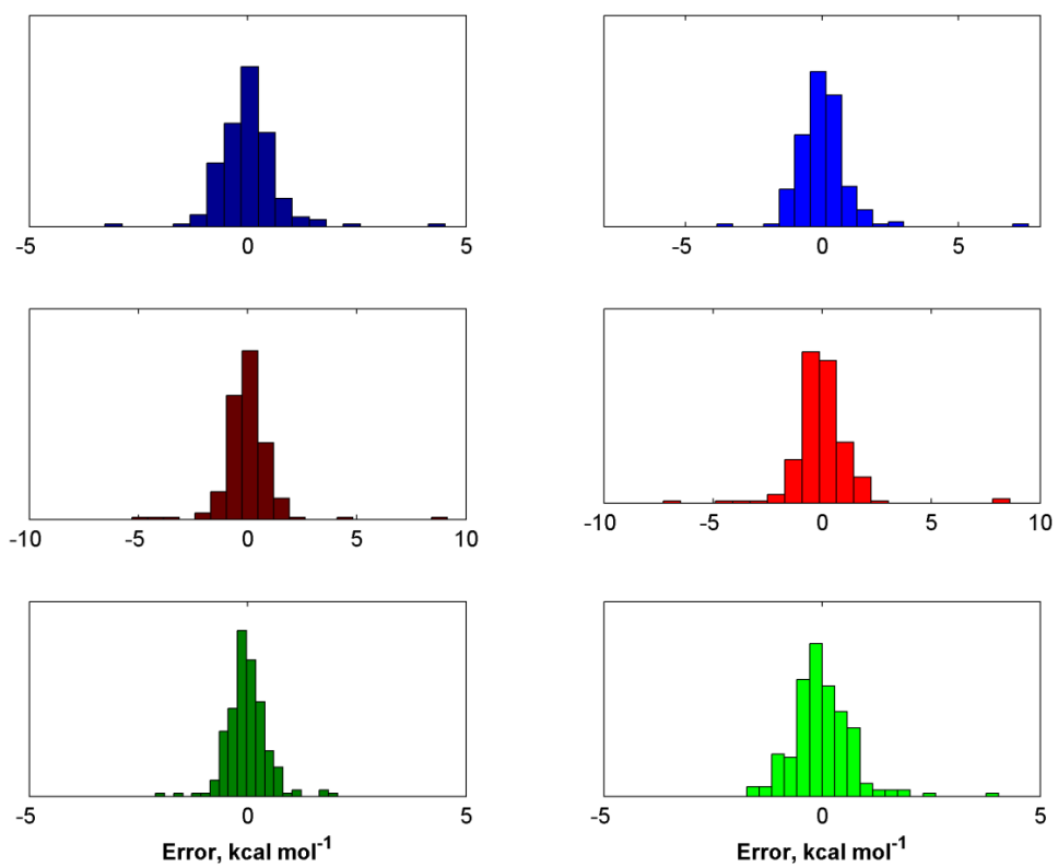
Figure S1. The error distributions for different DFT methods: (top) B3LYP, (middle) BLYP, (bottom) BMK; (left) 6-311(2df,2pd), (right) 6-311(3df,3pd).
