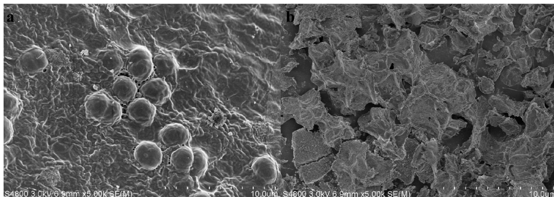
Fig. 6. SEM images of Microcystis aeruginosa treated by an aqueous extract of Artemisia argyria : (a) blank control (b) 15g/L after 10 days.
