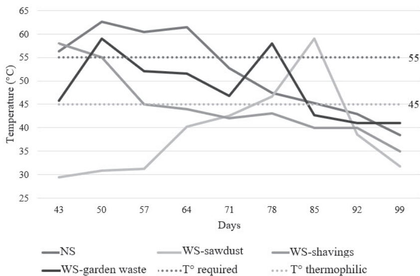
Fig. 8. Temperatures in the thermophilic phase with n = 3.
