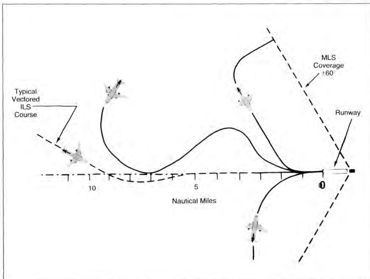
Map of vectors flown for research with the Microwave Landing System flight tests in 1978. Demonstrates three different curved paths possible instead of the straight line path used for ILS.
