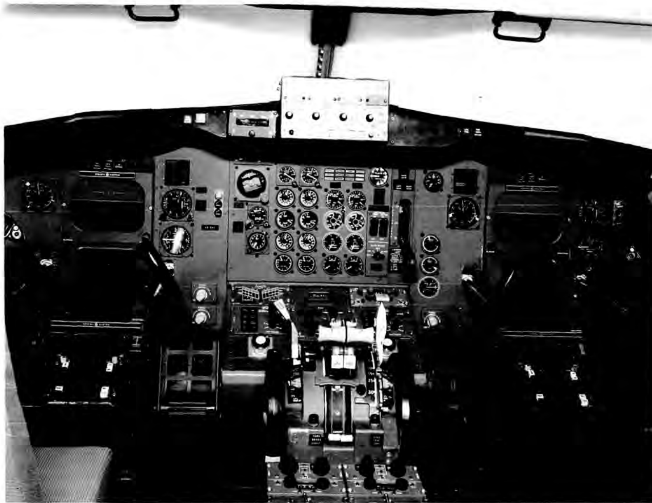
Original configuration of the aft flight deck of the NASA 737 with monochrome flight displays. Note the "Brolly Handle" flight controls.
