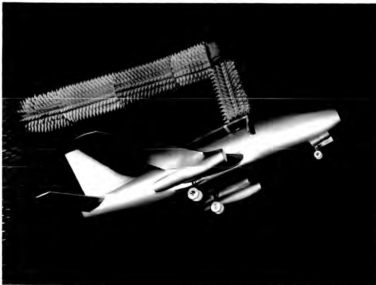
Wind tunnel model tests of placement of the antennae for Microwave Landing System research in 1974.
