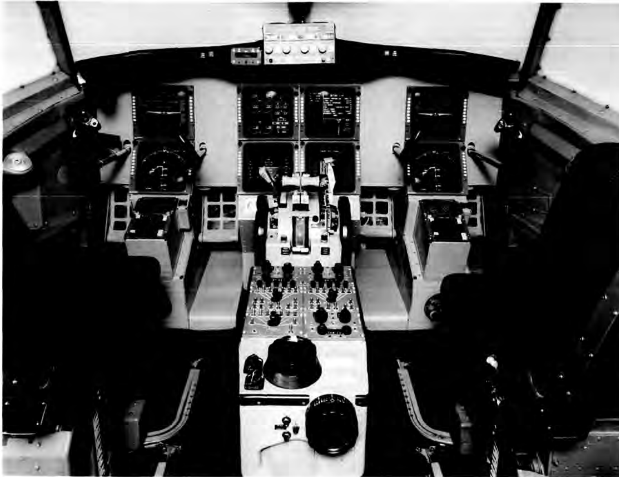
The aft flight deck of the NASA 737 in 1987. An upgrade in 1986 replaced four original 5 x 7 monochrome displays with eight 8 x 8 color monitors.
