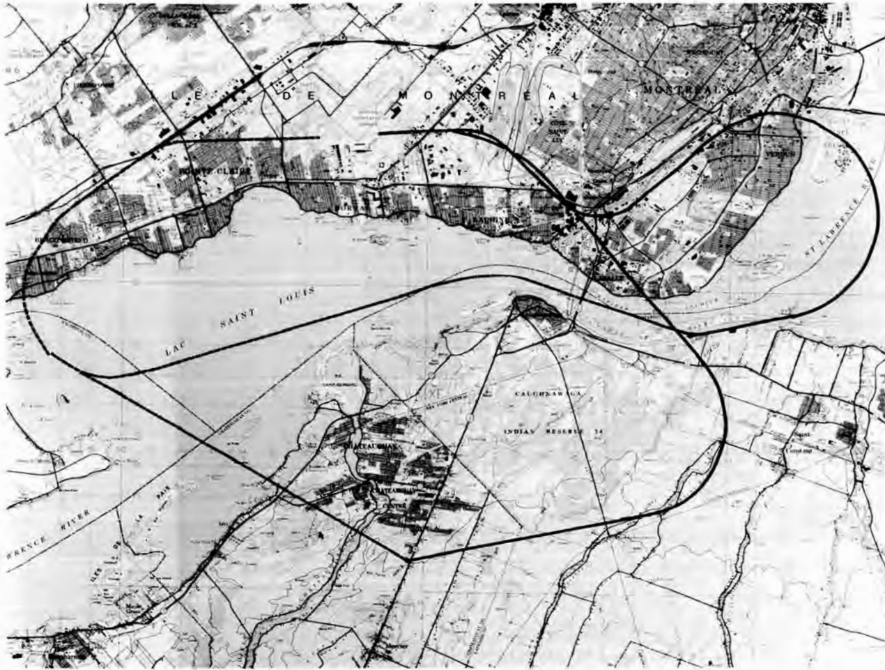
The Microwave Landing System flight demonstrations at Montreal, Canada. The map depicts two curved-path MLS approaches demonstrated by the Langley 737 during the 1978 ICAO meeting.
