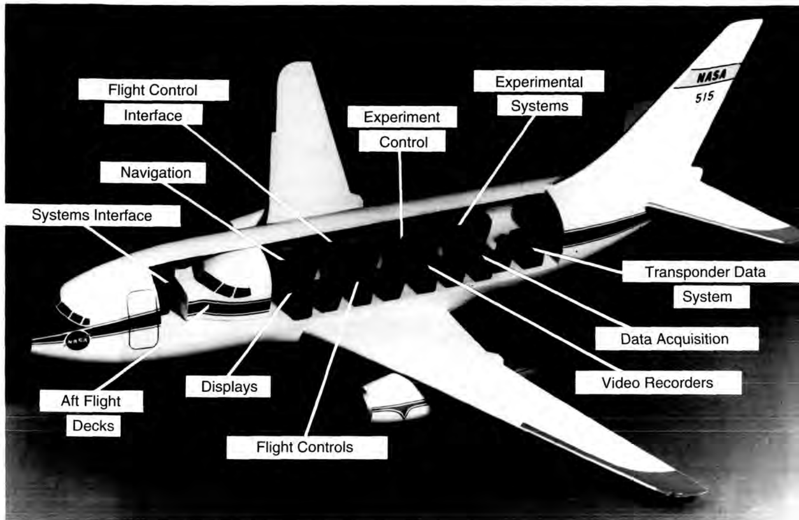
Cutaway model of the Boeing 737 used for flight research showing its aft cockpit and the location of various research pallets.
