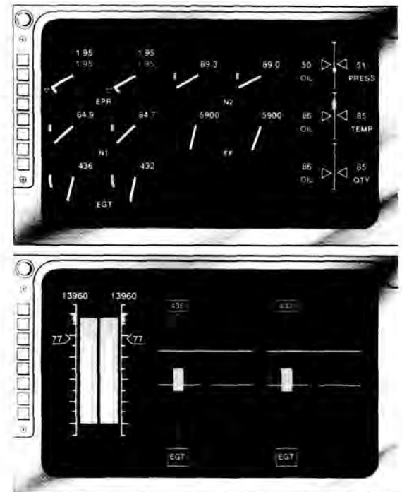
Displays of incorrect sensor readings during engine power-up for takeoff, similar to that experienced during the 1982 Air Florida accident at Washington National Airport. Top—Traditional display. Bottom—Engine monitoring and Control System (E-MACS) display. Note the visual superiority of E-MACS to warn flight crews of hazard.
