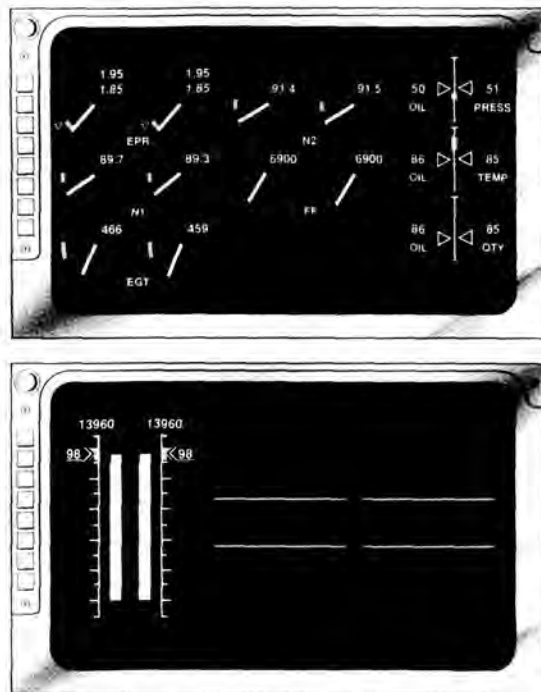
Displays of normal engine power-up for takeoff; top-traditional display, bottom-Engine Monitoring and Control System (E-MACS) display, designed for easy reading.
