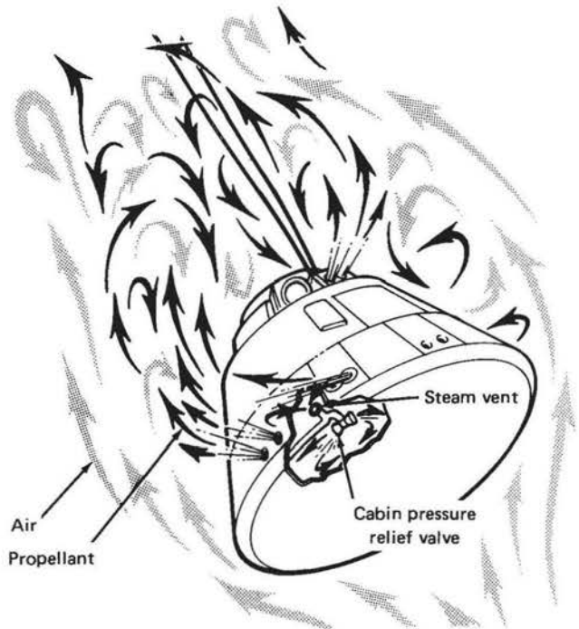
Diagram of air and propellant flow around the Apollo command module during descent through the atmosphere. Note propellant gases being drawn into the steam vent.
