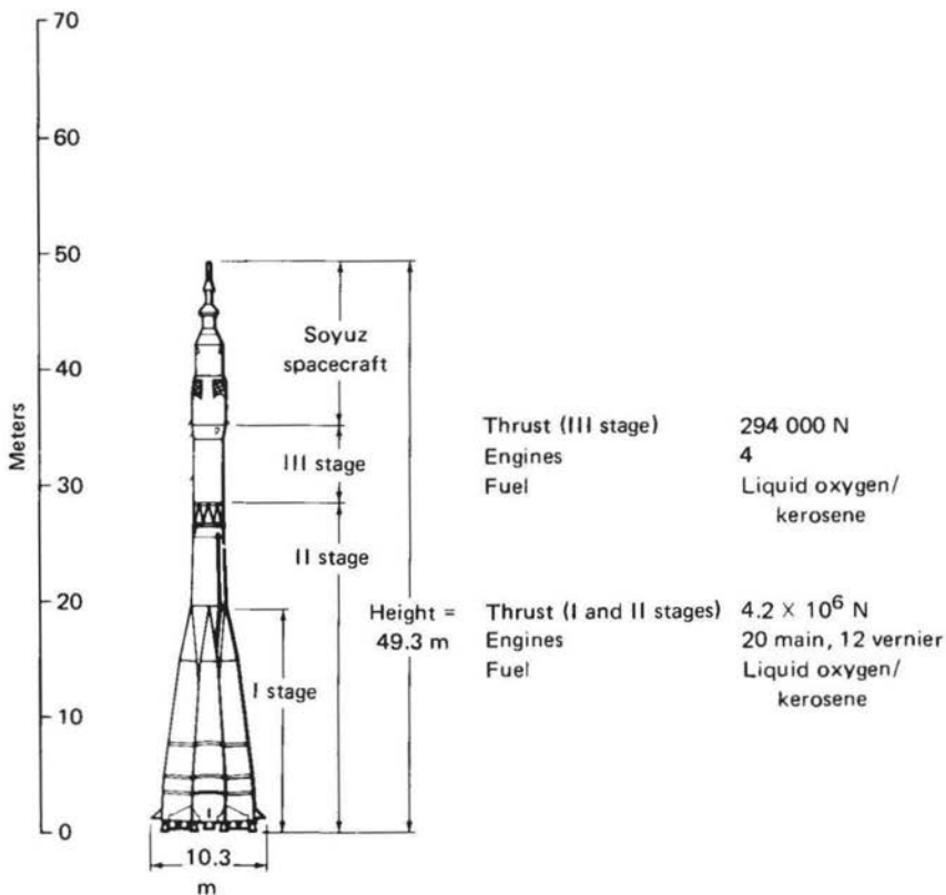
Soyuz launch configuration
