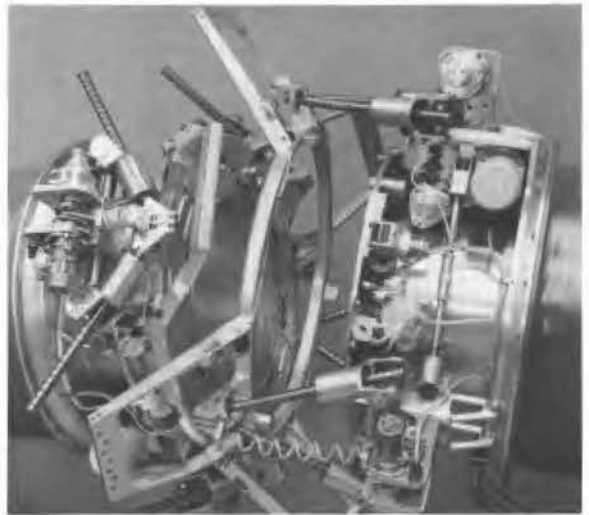
Two views of the Soviet two-fifths-scale model of their version of the ASTP docking system, used in the October 1972 Preliminary Systems Review in Moscow (Soviet Academy of Sciences photos).
