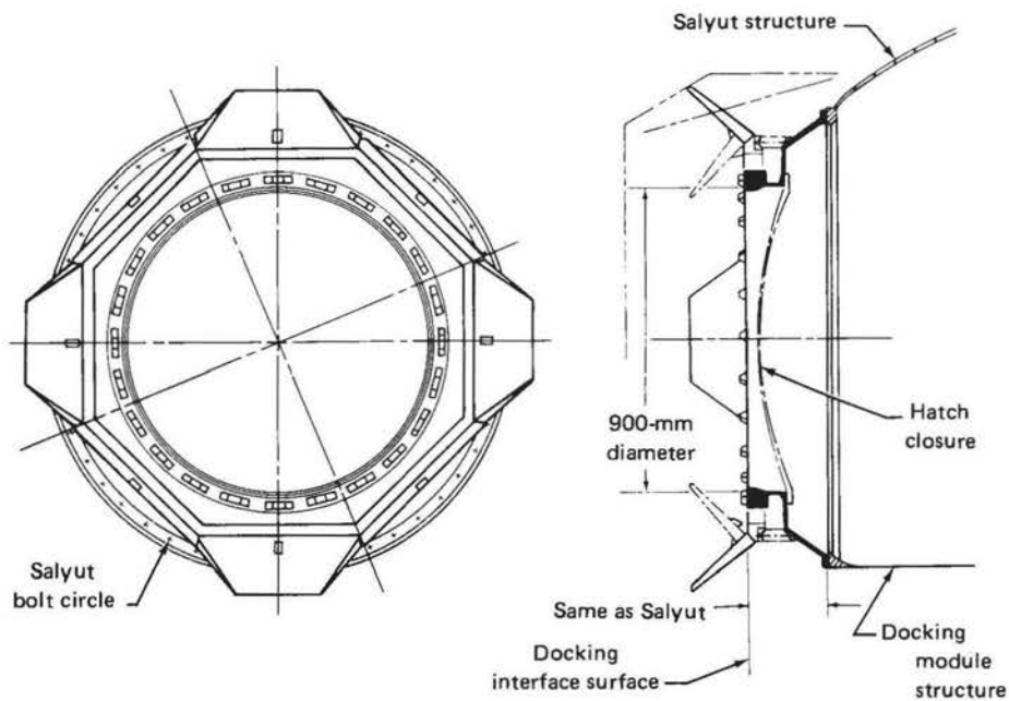
NASA proposal for a four-guide docking mechanism is shown to the Soviets during the November 1971 meeting in Moscow. Note the 900-millimeter-diameter tunnel.
