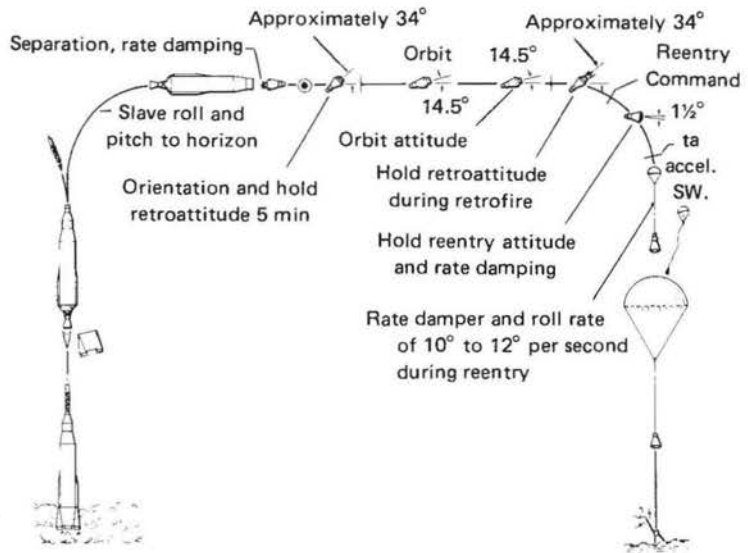
Typical mission profile for orbital Mercury flights.
