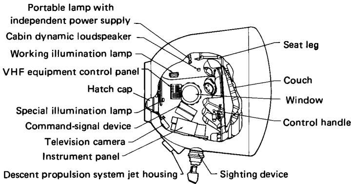
Soyuz descent vehicle.
