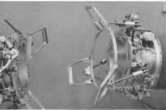
Two views of the Soviet two-fifths-scale model of their version of the ASTP docking system, used in the October 1972 Preliminary Systems Review in Moscow (Soviet Academy of Sciences photos).
