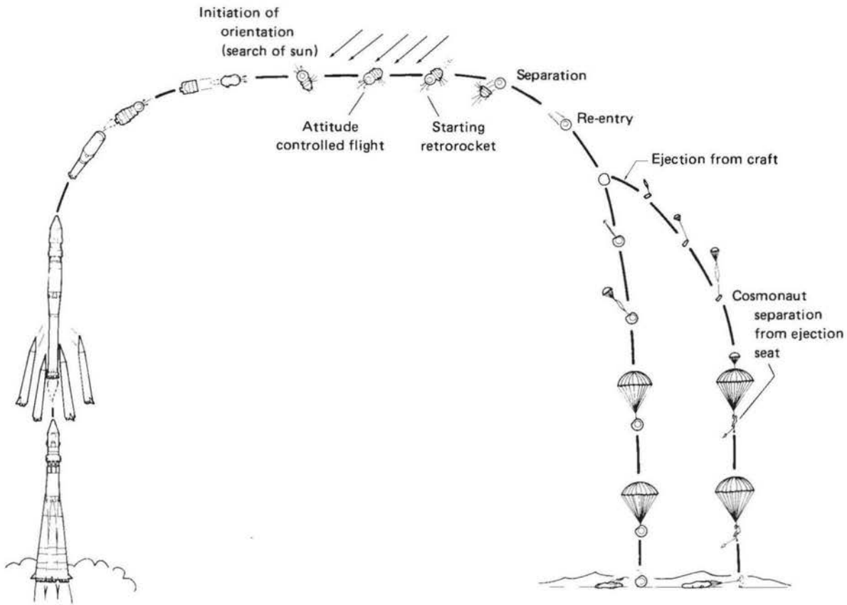
Typical mission profile for Vostok flights.
