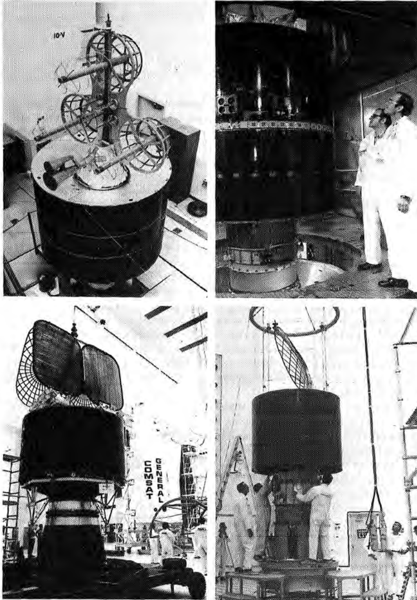
Four of the comsats in NASA's 1976 launch schedule: A, Comsat General's Marisat, launched 19 Feb.; B, NATO III-A, launched 22 Apr.; C, Comsat General's Comstar 1A, launched 13 May; D, Indonesia's Palapa, launched 8 July.
