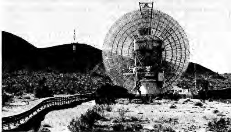
The 26-m "Venus dish" at NASA's Goldstone tracking station near Barstow, Calif., in use with rectenna (in background) for solar-energy conversion experiments. (NASA 76-H-685)
