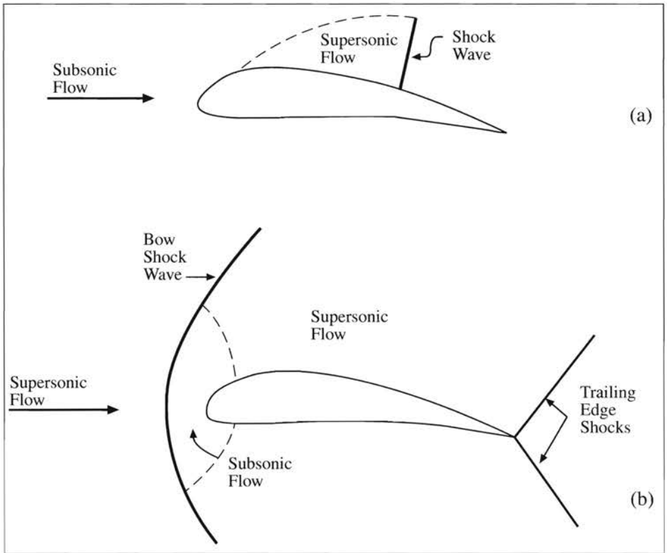
Schematic of transonic flow over an airfoil. (a) Freestream flow slightly below the speed of sound, typically a subsonic freestream Mach number from about 0.8 to 0.999. (b) Freestream flow slightly above the speed of sound, typically a supersonic freestream Mach number from 1.0 to about 1.2.
