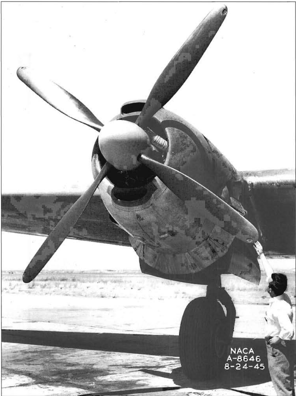
An air-heated propeller designed by Curtiss and installed on the NACA C-46. The heated air exhausted out the orifice at the tip of each blade. (NASA photo no. Ames A-8646).
