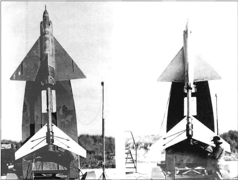
At Wallops Station, in tidewater Maryland, in 1953, Langley's Pilotless Aircraft Research Division (PARC) tested rocket-powered models of the delta-winged Convair F-102 before (left) and after (right) modification to take advantage of Whitcomb's "area rule." (NASA photo).
