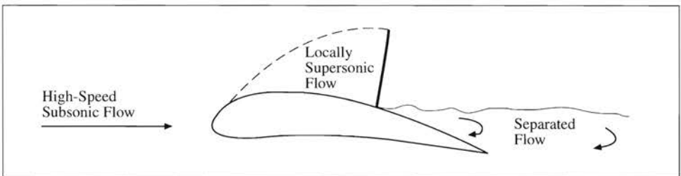
Schematic of shock-induced separated flow—the source of the compressibility burble.
