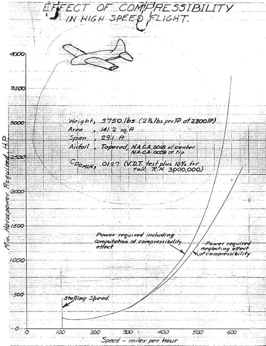
Graph and sketch hand-drawn by John Stack, 1933. The effect of compressibility on the power required for a hypothetical airplane. This sketch was subsequently sent to the October 1933 Committee Meeting of the NACA in Washington. From the John Stack papers at the NASA Langley Archives.
