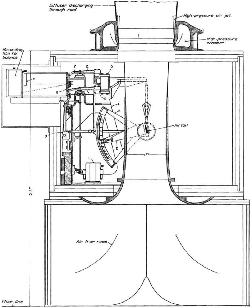
--Diagrammatic section of the high-speed wind tunnel.
