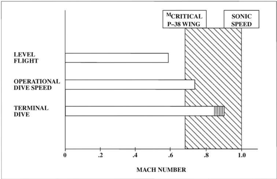
Bar chart showing the magnitude of how much the P-38 penetrated the compressibility regime.
