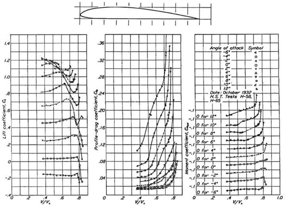
The first compressibility data published by John Stack. From NACA TR 463, 1933. The three graphs are, from left to right, the variations of lift coefficient, drag coefficient, and moment coefficient, respectively, versus the ratio of the freestream velocity to the speed of sound (the Mach number). The test model was a 3C1D airfoil, shown at the top of the figure. The adverse effects of compressibility are seen in the precipitous decrease in lift coefficient and dramatic increase in drag coefficient as the Mach number is increased.
