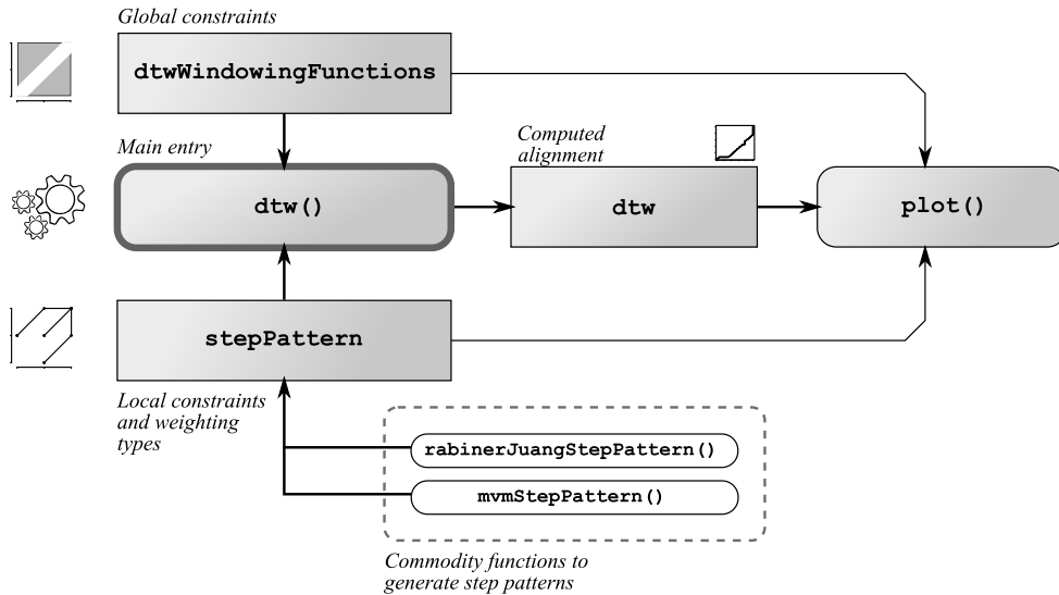
Figure 2: Block diagram of the main functions (rounded boxes) and object classes (rectangles) of the dtw package and their relationship. Arrows going in functions are arguments, outgoing are returned values.
