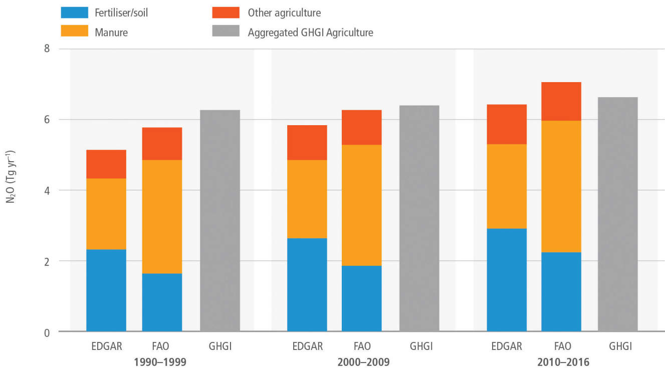
Figure 2.11 | Average agricultural N 2 O emissions estimates from 1990. Sub-sectoral agricultural emissions are based on the Emissions Database for Global Atmospheric Research (EDGAR v4.3.2; Janssens-Maenhout et al. 2017a); FAOSTAT (Tubiello et al. 2013) and National GHGI data (Grassi et al. 2018). GHGI data are aggregate values for the sector. Note that EDGAR data are complete only through 2012; the EDGAR data in the right-hand panel represent the three years 2010–2012 and are presented for comparison. FAO data for the “other agriculture” category includes emissions from crop residues, cultivated organic soil, and burning of crop residues.
