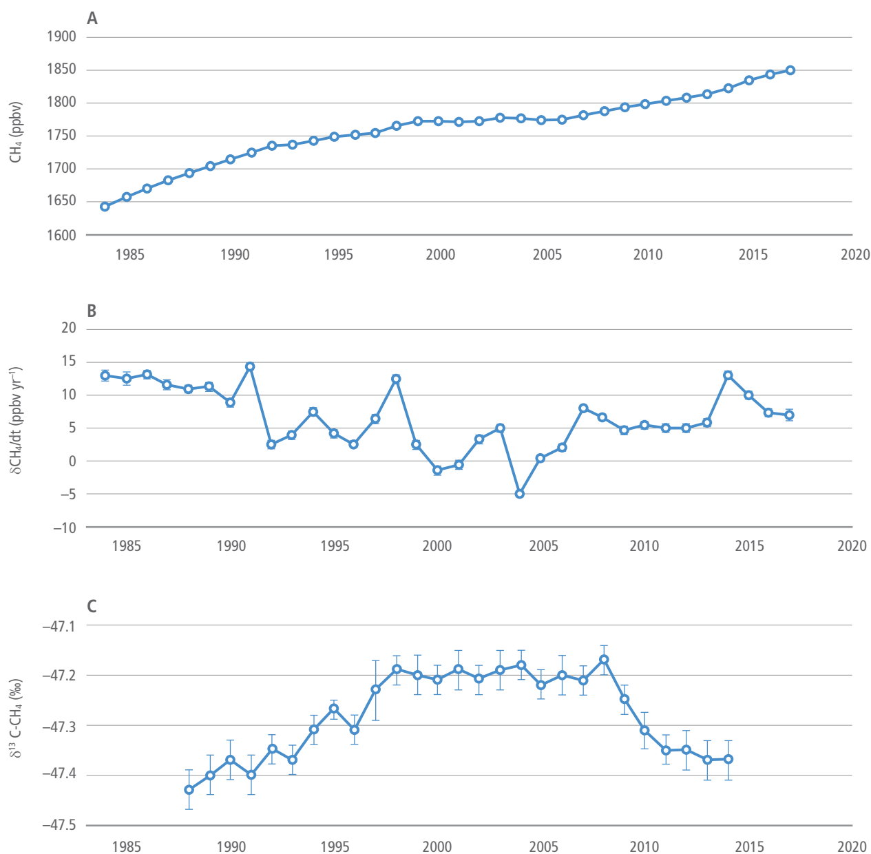
Figure 2.8 | Globally averaged atmospheric CH 4 mixing ratios (Frame A) and instantaneous rates of change (Frame B) and C isotope/variation (Frame C). Data sources: NOAA/ESRL ( www.esrl.noaa.gov/gmd/ccgg/trends_ch4 ); Dlugokencky et al. (1994) and Schaefer et al. (2016).
