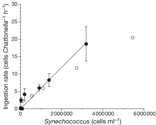
Fig. 7. Ingestion rate (IR) of Chattonella ovata (●) and C. subsalsa (○) on Synechococcus sp. as a function of initial prey concentration ( pc ). Data are mean \pm SE for C. ovata ( n = 3 for each prey concentration) and single treatments for C. subsalsa ( n = 1 for each prey concentration). The curve was fitted by a linear equation using all treatments in Expt 3 (for C. ovata ): IR = 5.66 \times 10^{-6} \times pc , r^2 = 0.668
