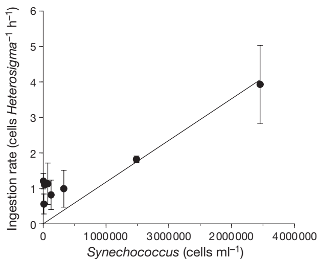
Fig. 8. Ingestion rate (IR) of Heterosigma akashiwo on Synechococcus sp. as a function of initial prey concentration ( pc ). Data are mean \pm SE. The curve was fitted by a linear equation using all treatments in the experiment: IR = 1.18 \times 10^{-6} \times pc , r^2 = 0.508
