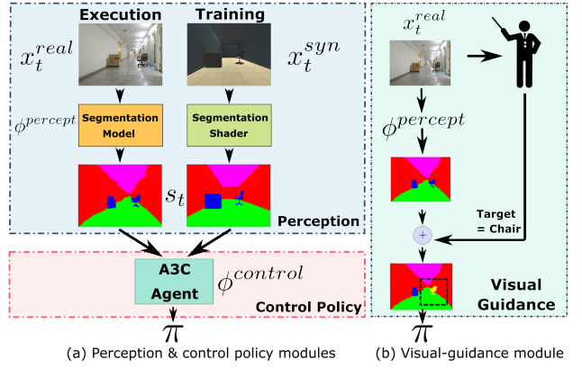
Figure 1: Model architecture
