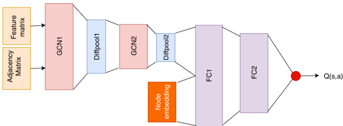
Figure 3: Geometric-DQN Architecture
