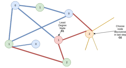
Figure 5: A toy example demonstrating observations O1 and O2 . The number on top of nodes denote the time-step at which they were discovered. Red nodes satisfy O1 . Orange nodes satisfy O2 . Green nodes are other potential actions. Blue denotes seed nodes
