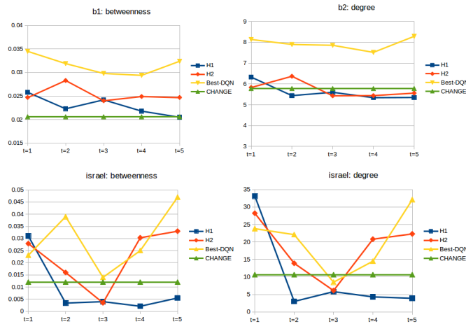
Figure 7: Average true betweenness(L) and degree(R) centrality across timesteps for H1, H2 and best Geometric-DQN. (We have added corresponding CHANGE values for reference)
