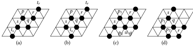
Figure 2: Configurations used in the proof of Theorem 3.1.
