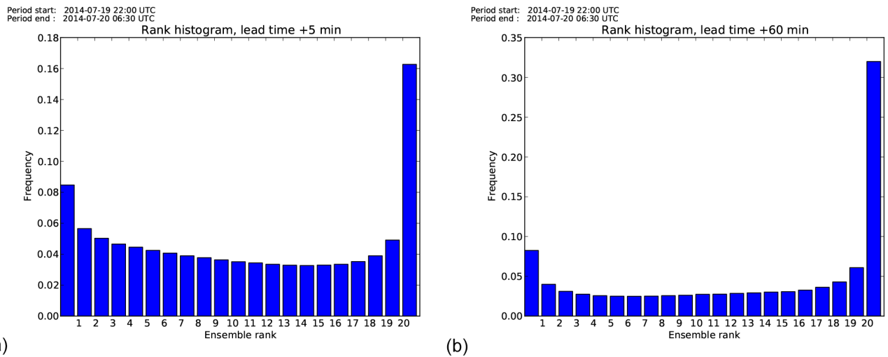
Figure 10. Rank histograms for the Leuven case on 19–20 July 2014 for a lead time of (a) 5 min and (b) 60 min.
