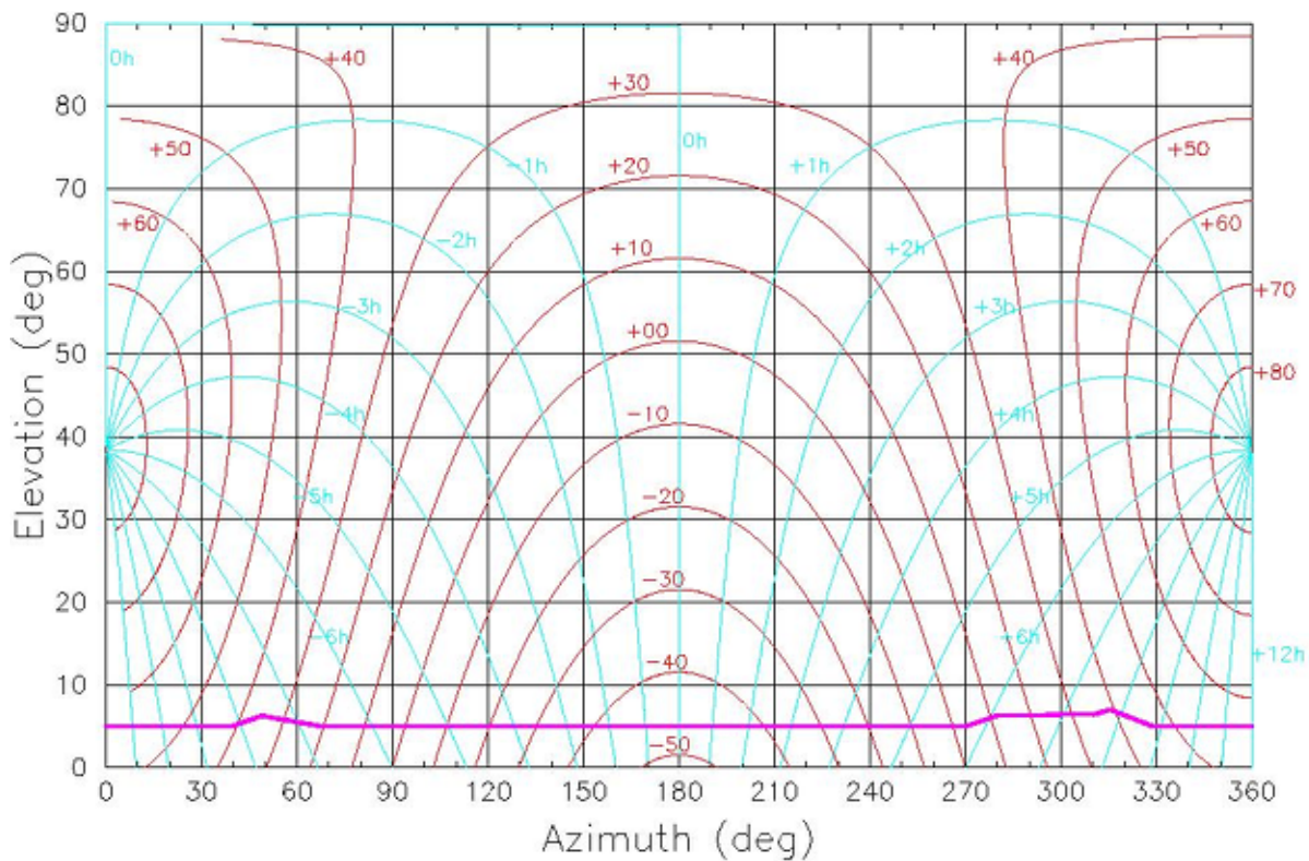
Figure 1: Plot of elevation vs azimuth, with lines of constant Hour Angle (HA; cyan lines) and Declination (DEC; brown lines) for the GBT. The horizon (magenta line) is shown at 5 degrees elevation, except for the mountains in the west and the 140-foot (43-m) telescope at azimuth = 48°. The lines of constant DEC are shown in increments of \pm 10^\circ , while the lines of constant HA are in increments of \pm 1 hour.
