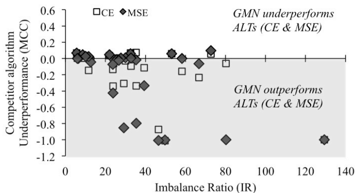
Fig. 1: Underperformance (measured by MCC) of both MSE and CE relative to GMN, plotted against imbalance ratio (IR). GMN outperforms the competitor cost functions everywhere in the shaded region.
