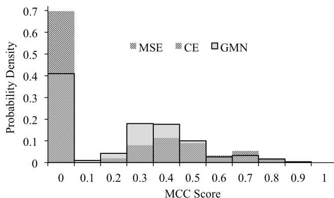
Fig. 2: Distribution of out-of-sample scores across all random seeds/ k -folds (300 total) for GMN, CE, and MSE cost functions, for the exceptional dataset abalone-20_vs_8-9-10 .
