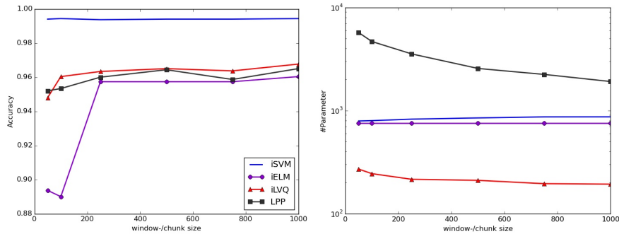
Fig. 1: Influence of the window-/chunk size on the accuracy (left) and model complexity (right) for dataset Border .
