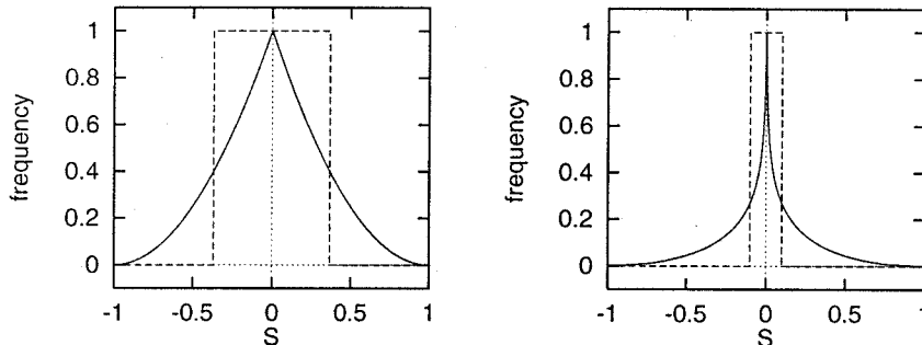
Figure 2: Left: Optimal 'tuning curves': long times (full curve), short times (dashed curve). Right: Optimal 'tuning curves' with constraint \mu = 0.1 : long times (full curve), short times (dashed curve).
