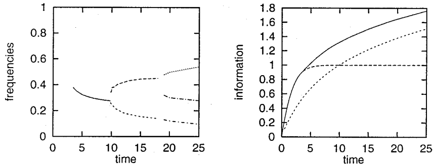
Figure 1: Left: Frequencies of the optimal distribution as a function of time. Right: Information capacity of the spiking neuron as a function of time (full curve); information transmitted in the case of a binary distribution (long-dashed curve); information transmitted in the case of the long-time optimal distribution (short-dashed curve)
