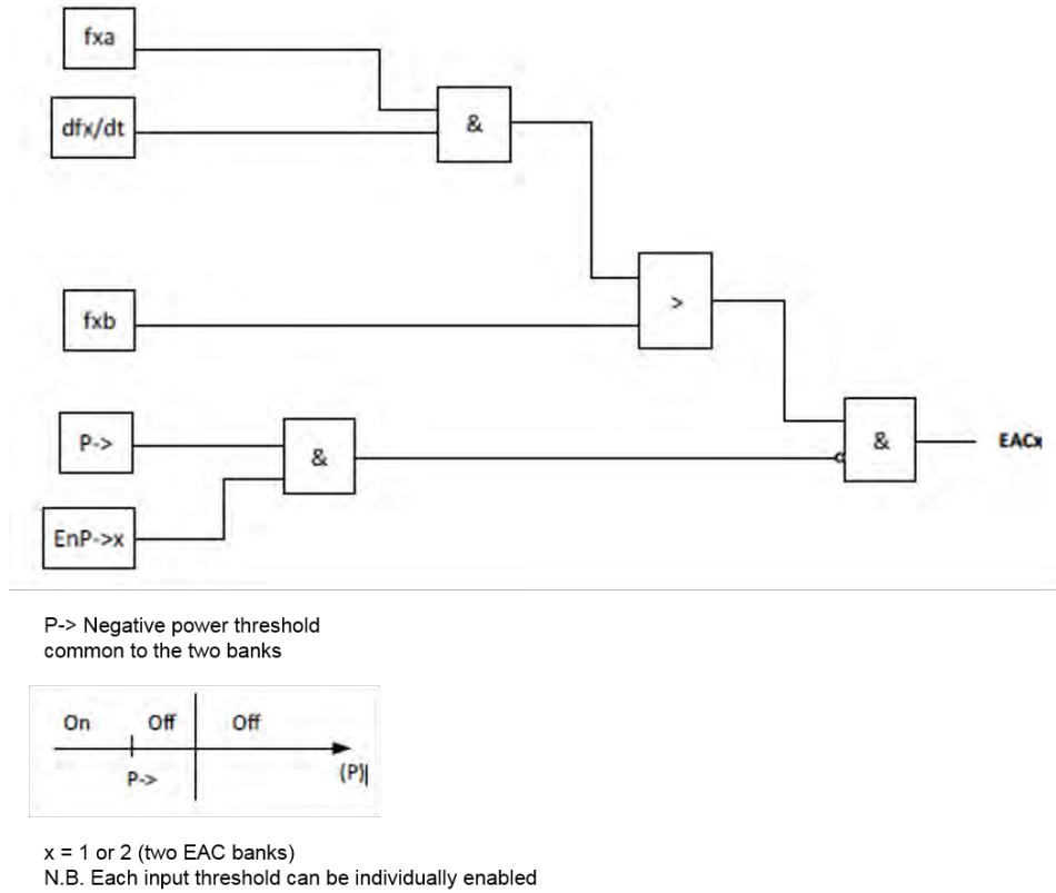
Figure 43 – EAC Logic
