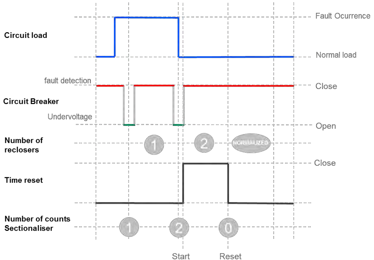
Figure 55 - Reset Counter
