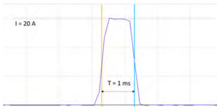
Figure 67 – Impulse test, T = 1 \text{ ms}
