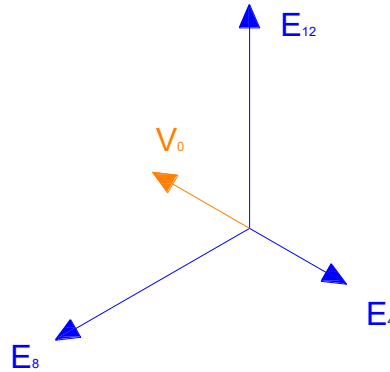
Figure 29 – Residual Voltage
