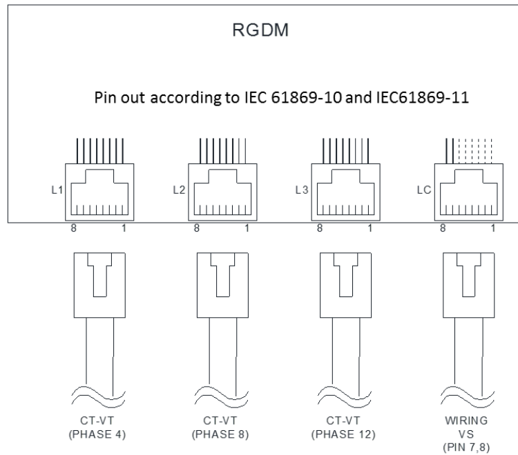
Figure 7 – Extended configuration
