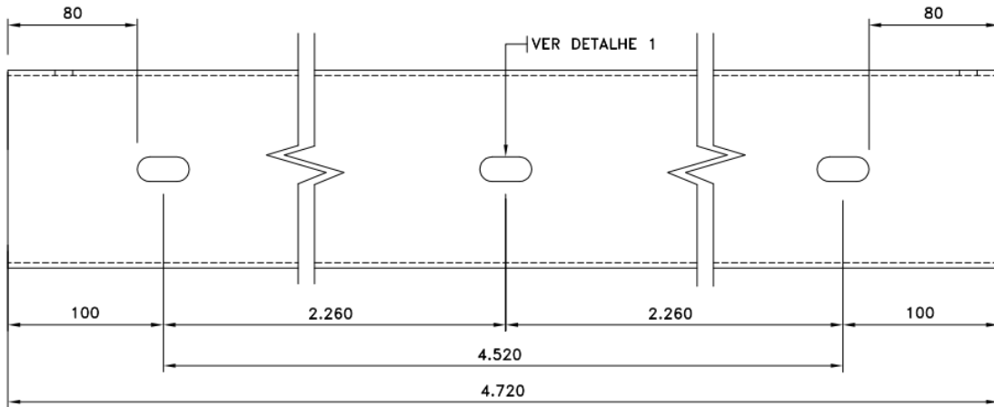
VISTA FRONTAL
