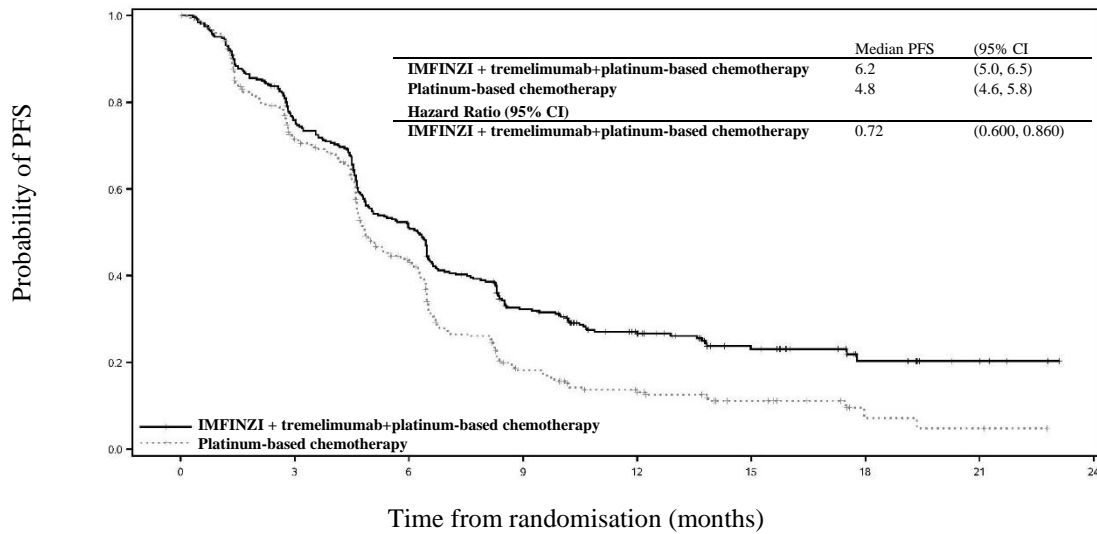
Figure 8. Kaplan-Meier curve of PFS
