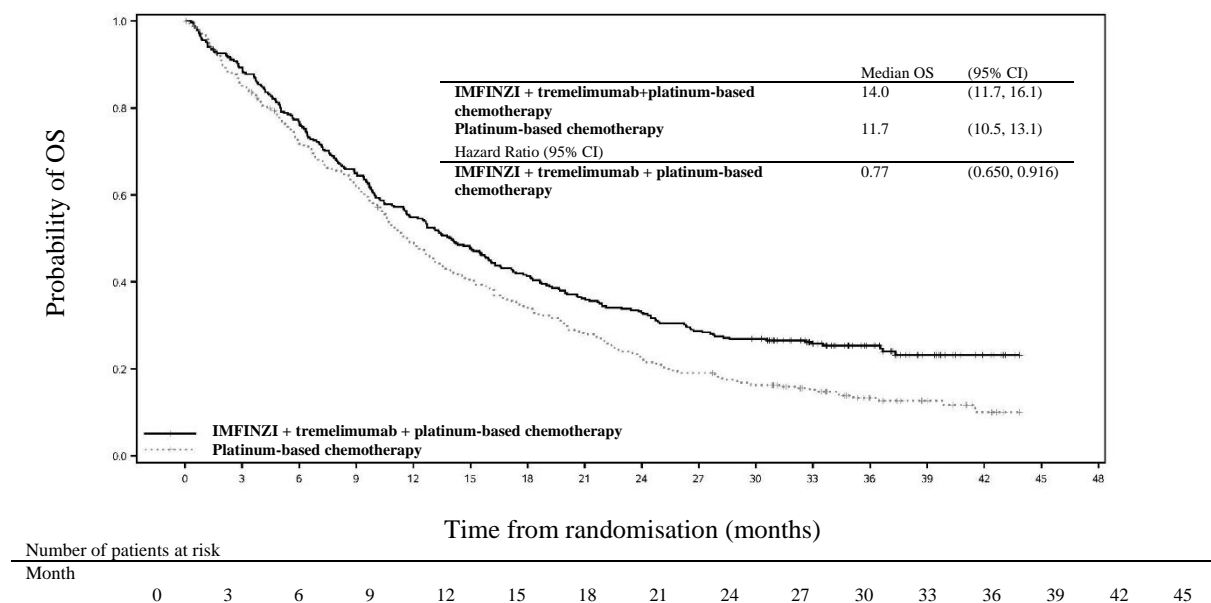
Figure 7. Kaplan-Meier curve of OS
