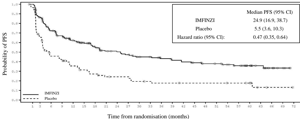
Figure 4. Kaplan-Meier curve of PFS for PD-L1 TC ≥ 1%
