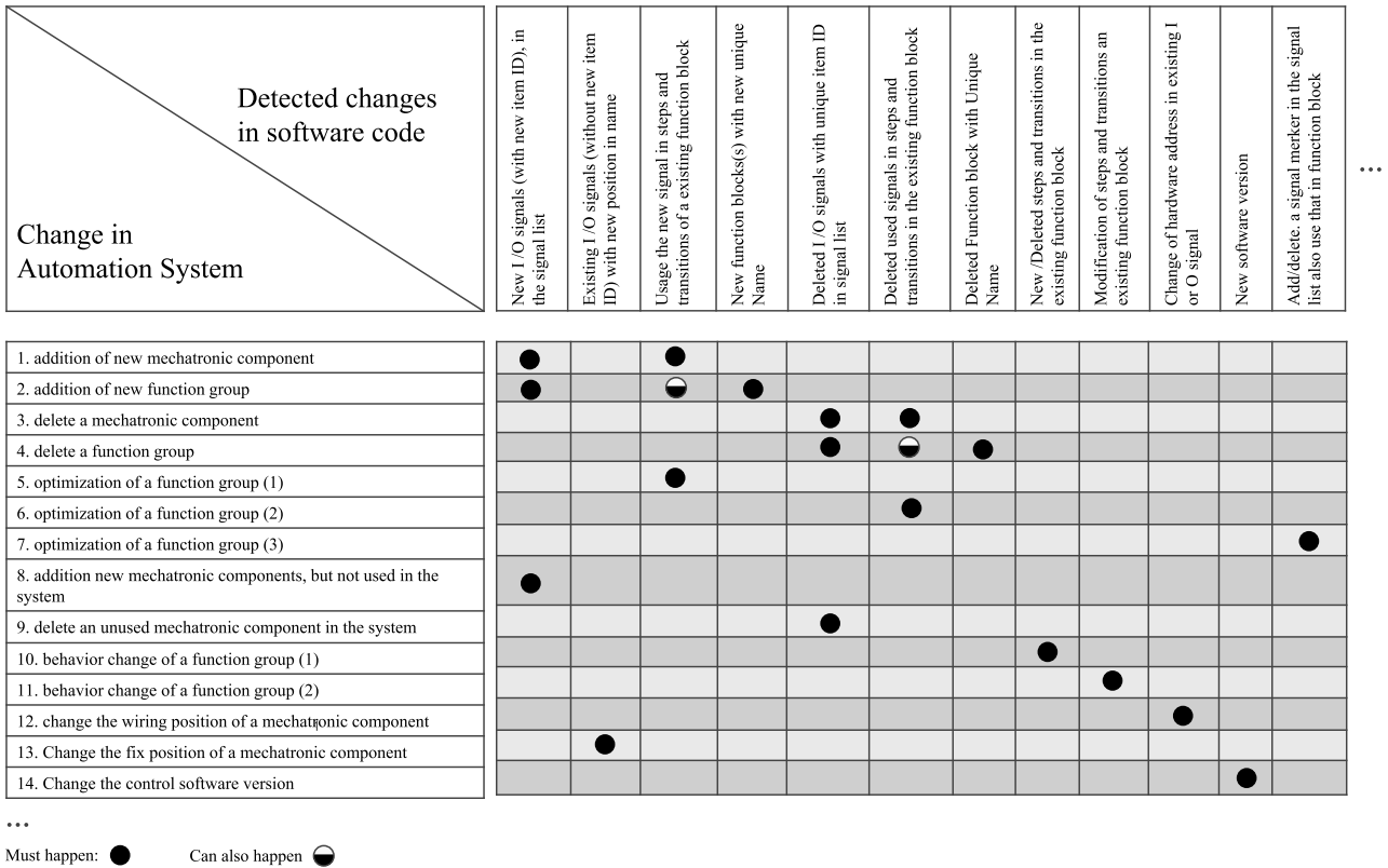
Figure 6: Rules table for rule-based change detection in automation systems.
