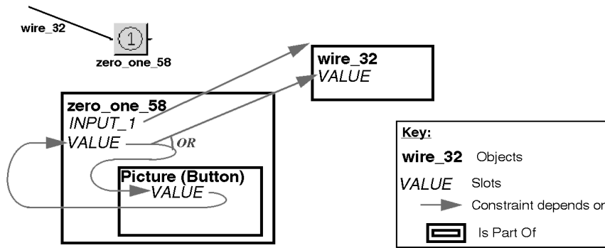
Fig. 4. The VALUE slot of the zero_one objects have a constraint that depends on either the value of the input wire, if it exists, or else the value of the button if there is no wire (if the INPUT1 slot is NULL ). The button in the PICTURE slot has a constraint that depends on the value for the zero_one object so it will have the right value when there is a wire. This creates a cycle of constraints.
