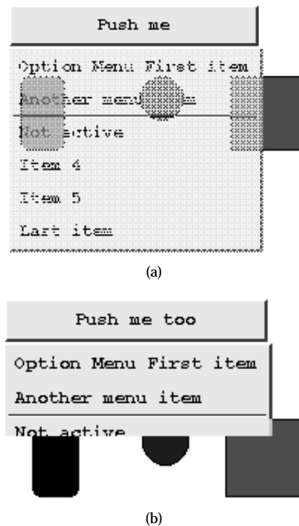
Fig. 5. Animation constraints can be added to the Am_VISIBLE slot of a pop-up menu to make it (a) fade in using halftoning; or (b) grow from the top.
