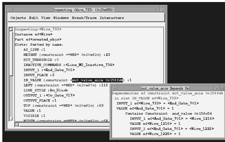
Fig. 11. Inspecting a wire in the circuit program, and the constraint in its IN_VALUE slot. The slots which are inherited are shown in blue on the screen. Notice that the high-level names are shown for methods, constraints and objects.
