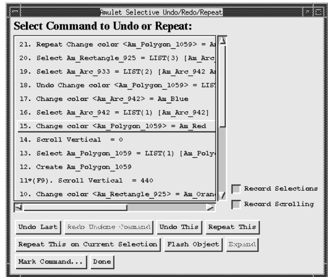
Fig. 10. The experimental dialog box that allows users to access the regular undo and redo operations (the first two buttons below the scrolling list). Other buttons operate on the command selected in the list (here, number 15), and will undo it, repeat it, or repeat it on new objects. "Flash Object" shows the object associated with the command. The "Expand" button will allow a command which operates on multiple objects to be separated into separate commands. Commands can be "marked" to allow them to be repeated with a single keystroke. Command 11 has been marked with the F9 keyboard key as an accelerator. The display of each command shows the action, the name of the objects affected, and the new value. The radio buttons on the right cause scrolling and selection commands to be queued, so that, for example, an accidental deselection of a set of objects can be undone.
