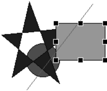
Fig. 7. A collection of Opal objects. The color of the star can be changed by simply setting its Am_FILL_STYLE slot, and Amulet will redraw the star and the other objects that overlap it. The Amulet toolkit includes selection handles shown around the rectangle which support selecting, moving and growing one or more objects.
