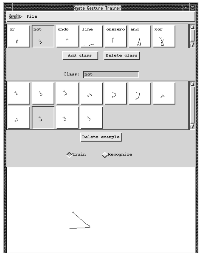
Fig. 8. The Agate interactive tool allows gestures to be created by example. Here, the gesture set for the circuit program is shown. A file is written describing the gestures which will then be read by a gesture interactor and used in applications. "Agate" stands for A G esture-recognition A nd T rainer by E xample and is based on a similar tool in Garnet [14].
