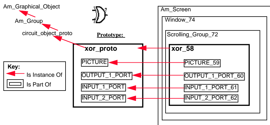
Fig. 3. The xor_proto object contains four parts: a bitmap called PICTURE , and output and input ports which are instances of lines. The xor_proto object is an instance of the circuit_object_proto object, which in turn is an instance of an Am_Group , which is an Am_Graphical_Object . When an instance is made of the xor_proto , Amulet automatically creates instances of each of the parts. If instances are not named, then Amulet makes up a name by appending a number. The instance, called xor_58 , has been made a part of a scrolling group, which is part of a window, which is part of the screen, so it will be visible.
