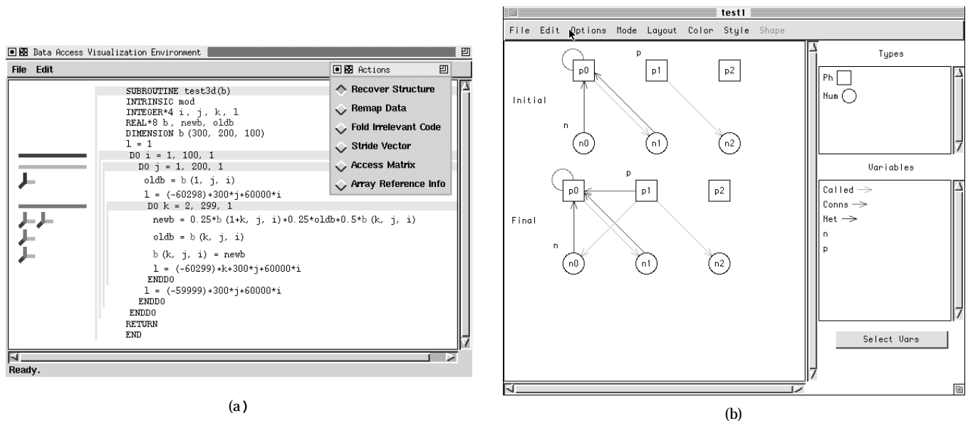
Fig. 12. Examples of two applications built using Amulet. (a) The Data Access Visualization Environment, a program designed to aid programmers in optimizing and parallelizing Fortran programs. (Courtesy of Galen C. Hunt, Computer Science Department, University of Rochester.) (b) A system to visualize the counter-examples discovered by the Nitpick analyzer for software specifications in Z, created as a class project by Craig Damon and Geoff Langdale at CMU. Many others are shown on the Amulet web pages at http://www.cs.cmu.edu/amulet/amulet-users.html .
