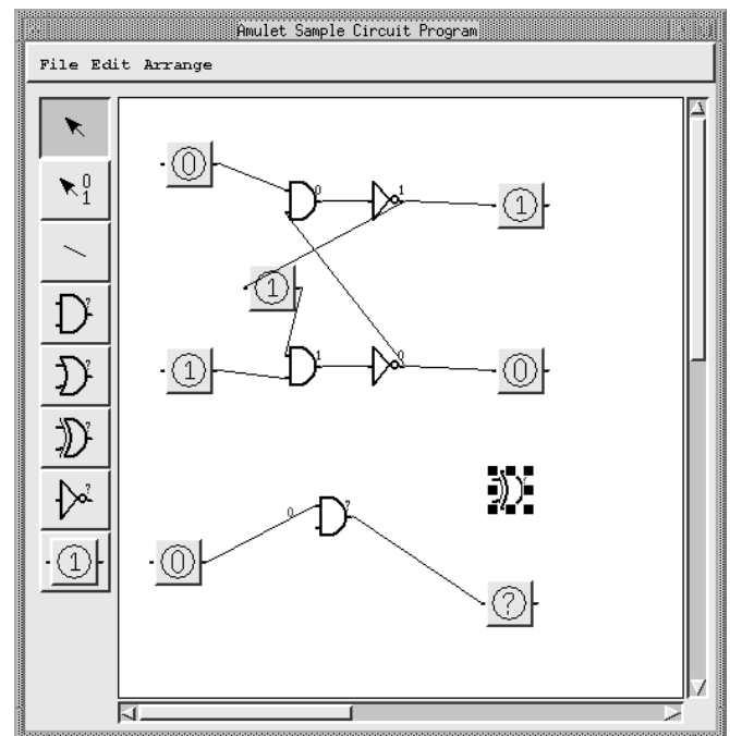
Fig. 1. A simple circuit design program created with Amulet.
