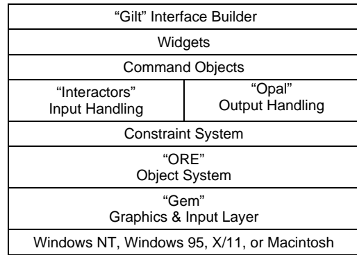
Fig. 2. The overall structure of the Amulet system.
