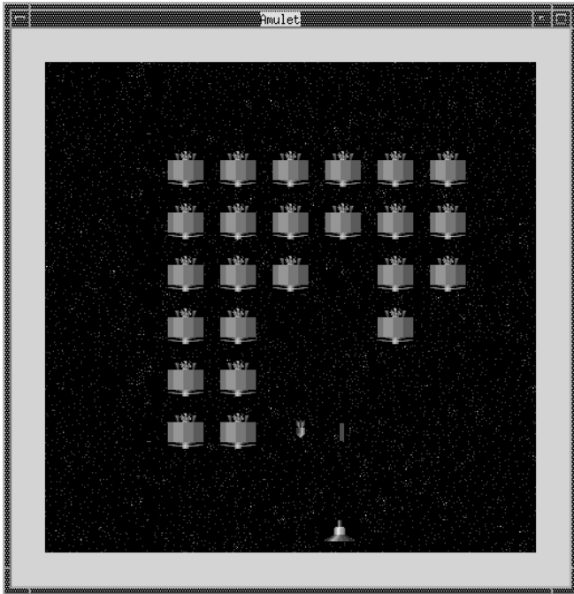
Fig. 6. The ships, bullets, and bombs are controlled by simple animators. For example, the bullets can be sent to the top of the screen by simply attaching an animation constraint to their AM_TOP slot and then setting that slot to -10 .
