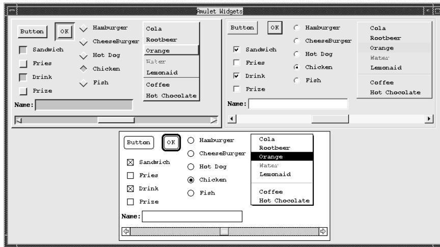
Fig. 9. Some of the widgets in Amulet with the Motif, Windows 95, and Macintosh look-and-feel in a window running under Motif. All of the widgets are implemented using Amulet intrinsics, and the choice of the look-and-feel is controlled by a slot which defaults to an appropriate value for the particular machine but can also be set explicitly.
