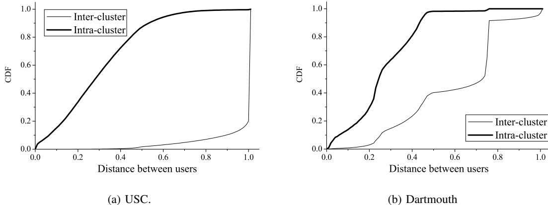
Fig. 3. Cumulative distribution function of distances for inter-cluster and intra-cluster user pairs (AMVD distance).
