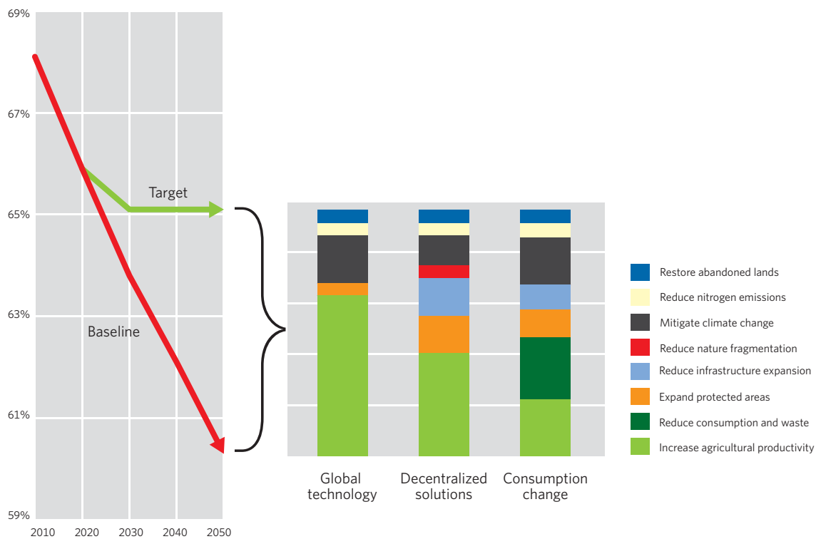
Figure 21.5. Contrasting pathways to sustainability using the Rio+20 socio-economic scenarios. The scenarios illustrated here would each reach by 2050 the goals of slowing and eventually halting biodiversity loss, while also keeping global average temperature increases within two degrees Celsius and achieving a range of socioeconomic development goals including ending hunger and providing universal access to safe drinking water, basic sanitation and modern energy sources. The goals can be reached by three different pathways (see Box 21.1).
