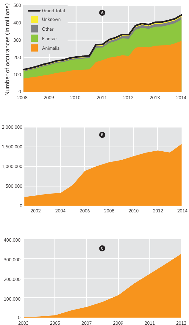
Figure 19.1. Growth in A species occurrence records published through the Global Biodiversity Information Facility, 224 B species covered in the Catalogue of Life annual checklist 225 and C number of animal species represented in the Barcode of Life Data Systems global reference library. 226
