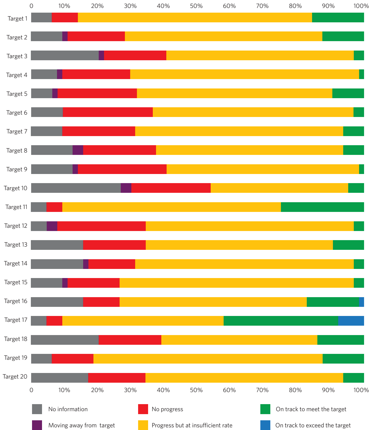
Figure 21.2. Assessment of progress towards the attainment of the Aichi Biodiversity Targets based on the information contained in 64 fifth national reports. 242 Almost 60 per cent of these reports explicitly assessed national progress towards the Aichi Biodiversity Targets. Where this is the case, the country's assessment has been applied to the same five point scale used in the target 'dashboard' shown on page 18 of this report. In the other cases the assessment has been inferred from the information contained in the report. A number of these reports did not contain information that allowed for an assessment of progress. These cases are represented in the figure as "No Information".
