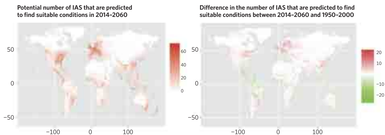
Figure 9.3. Projected changes in the occurrence of invasive alien species due to climate change based on species distribution models and future projections of climate and land use change. 142
