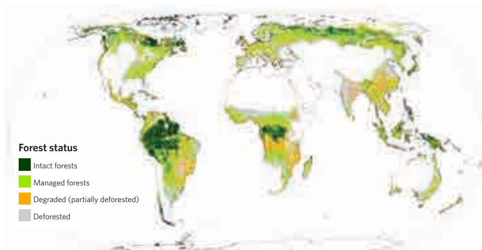
Figure 5.1. The extent of deforestation and forest degradation worldwide. 69 Intact forests refers to unbroken expanses of natural ecosystems greater than 50,000 hectares. Managed forests refers to forest that is fragmented by roads and/or managed for wood production. Degraded or partially deforested refers to landscapes where there has been a significant decrease in tree canopy density. Deforested refers to previously forested landscapes which have been converted into non-forest.
