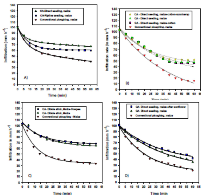
Figure 6.2. Infiltration rate in mm h -1 measured with a rainfall simulator in different CA and one conventionally tilled treatment at Henderson Research Station, Zimbabwe (A), Monze, Farmer Training Centre (B), Chitedze Research Station (C) and Sussundenga Research Station (D), January 2010 (Thierfelder, 2011, unpublished data).
