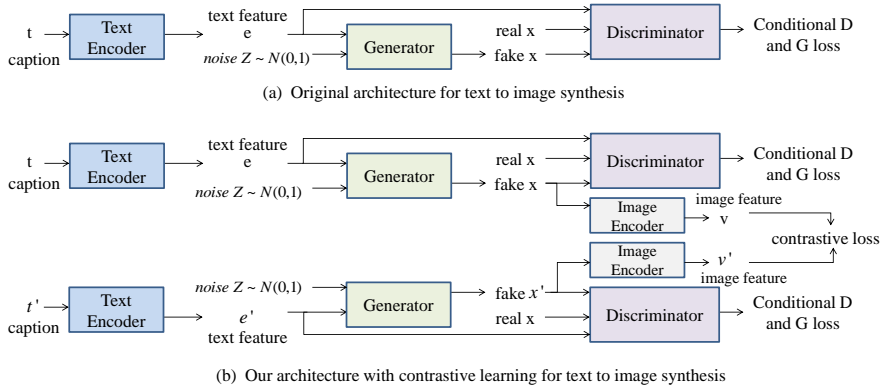
Figure 2: Architectures of original approach and our approach for text to image synthesis.
