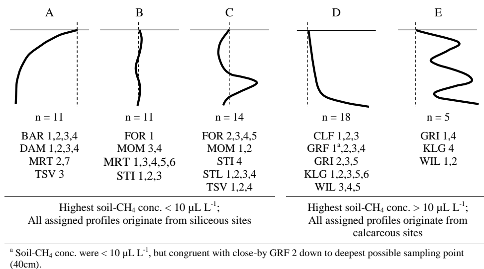
Fig. 5. Qualitative categories A–E assigned to measured soil-gas CH 4 profiles according to profile appearance. Illustrated profile shapes are typical for each category. The vertical line indicates atmospheric CH 4 concentration. Sampled locations assigned to the respective categories are listed below.
