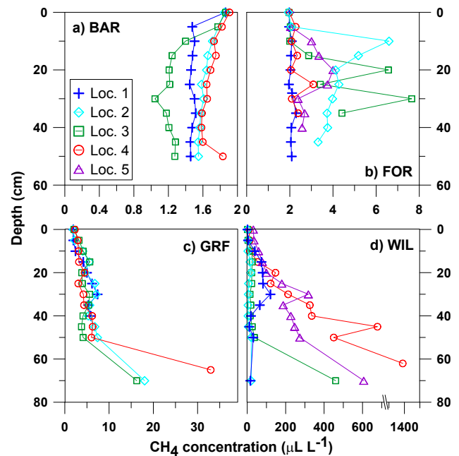
Fig. 1. Selection of measured soil-gas CH 4 concentration profiles representative for the different situations encountered. The legend in plot (a) applies to all subplots. Note the different scale in CH 4 concentrations for each site.
