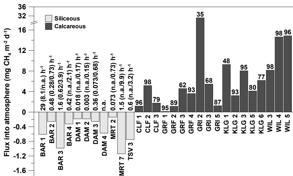
Fig. 2. Fluxes of CH 4 from the soil into the atmosphere ( J_{\text{atm}} ) for locations where the profile shape allowed quantification. Negative J_{\text{atm}} indicate that the soil was a sink for atmospheric CH 4 . For these locations estimated k of CH 4 oxidation are reported (with low/high 95 % confidence interval). For locations with positive J_{\text{atm}} , the number above the bars indicates the percentage of CH 4 oxidized in the soil before reaching the atmosphere. Note that the scale for negative and positive fluxes is different.
