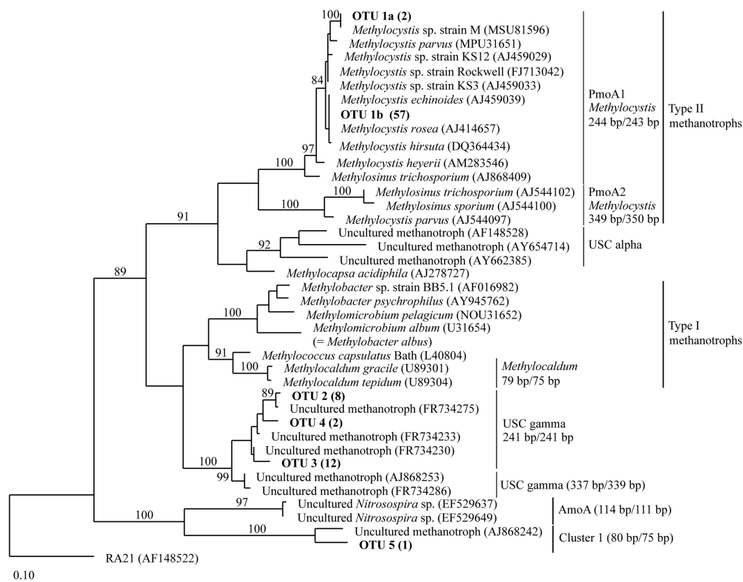
Fig. 3. Maximum likelihood tree showing the phylogenetic affiliation of pmoA sequences obtained from different glacier forefields. The pmoA tree was constructed based on 139 derived amino acid sequence positions. The neighbor-joining method resulted in essentially the same tree topology. Sequences obtained in the course of this study were grouped into 5 species-level units (OTU 1 to 5) based on an amino acid sequence identity threshold of 93 %. The number of clones obtained for each OTU is given in parentheses. All species-level OTUs also contain published pmoA sequences. Predicted T-RF lengths based on MspI are shown on the left side, while the experimental T-RF lengths are indicated on the right side. The in silico predicted T-RF lengths were experimentally confirmed by T-RFLP analysis of individual pmoA clone sequences. Bootstrap values greater than 80 are shown (100 replicates). The sequence of RA21 (AF148522) was used as outgroup. The scale bar represents 10 % sequence divergence or 0.1 substitutions per amino acid position.
