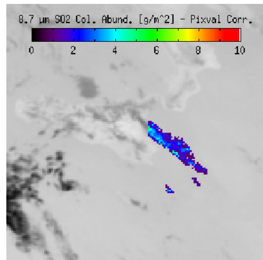
Fig. 15. 24 November 2006 SEVIRI image 12:15 UTC. Ash correction for 8.7 \mu\text{m} SO 2 retrieval. Top plate: meanval procedure. Bottom plate: pixval procedure.
