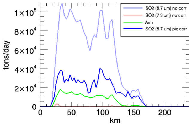
Fig. 16. SO 2 and ash flux derived from the SEVIRI image. The pale red and pale blue lines represents the SO 2 flux at 7.3 and 8.7 μm respectively before the correction, the red and blue lines represents the SO 2 flux at 7.3 and 8.7 μm after the pixval correction and the green line is the ash flux.
