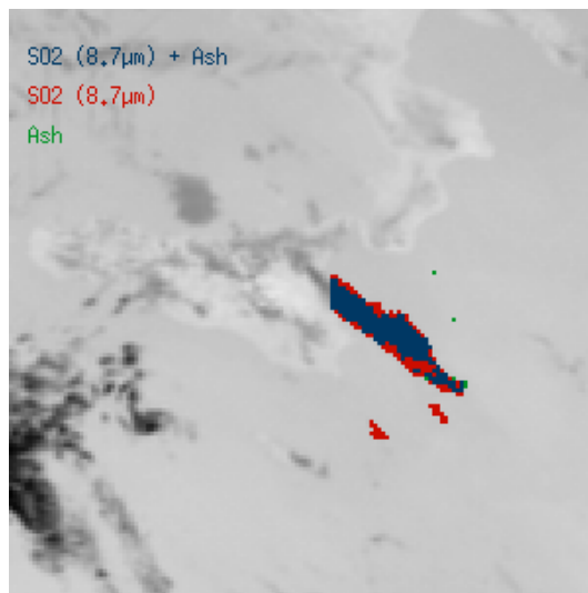
Fig. 14. 24 November 2006 SEVIRI image 12:15 UTC ensemble intersection. Top plate: intersection between ash and SO 2 at 7.3 \mu\text{m} ensembles. Bottom plate: intersection between ash and SO 2 at 8.7 \mu\text{m} ensembles.
