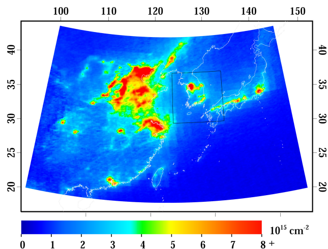
Figure 1. Warm-season averaged (May–September) NO 2 tropospheric vertical column content using the OMI-standard NO 2 product for the years 2015–2017 in East Asia. The 4 km × 4 km WRF-Chem domain is outlined over the Korean Peninsula.
