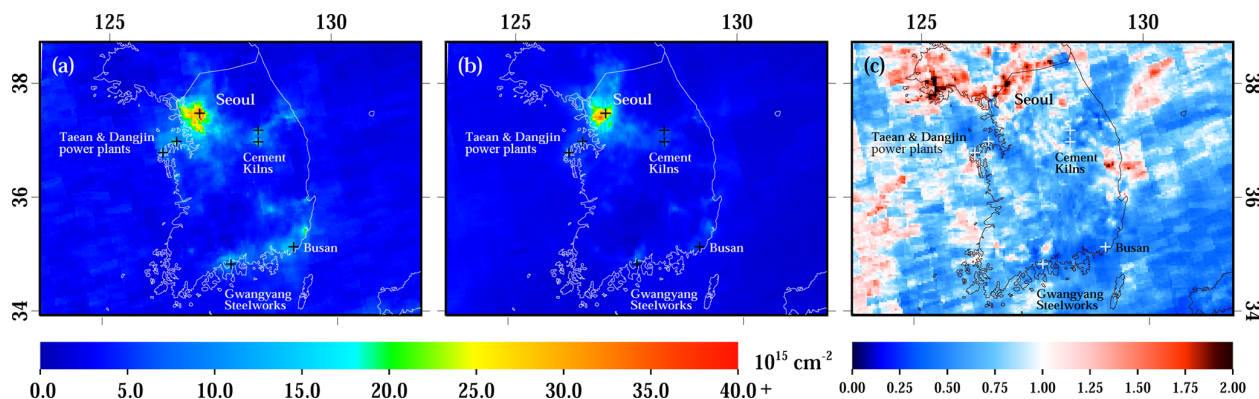
Figure 10. Same as Fig. 3, but now showing the WRF-Chem simulation with NO x emissions in the Seoul metropolitan area increased by a factor of 2.13 in panel (b).
