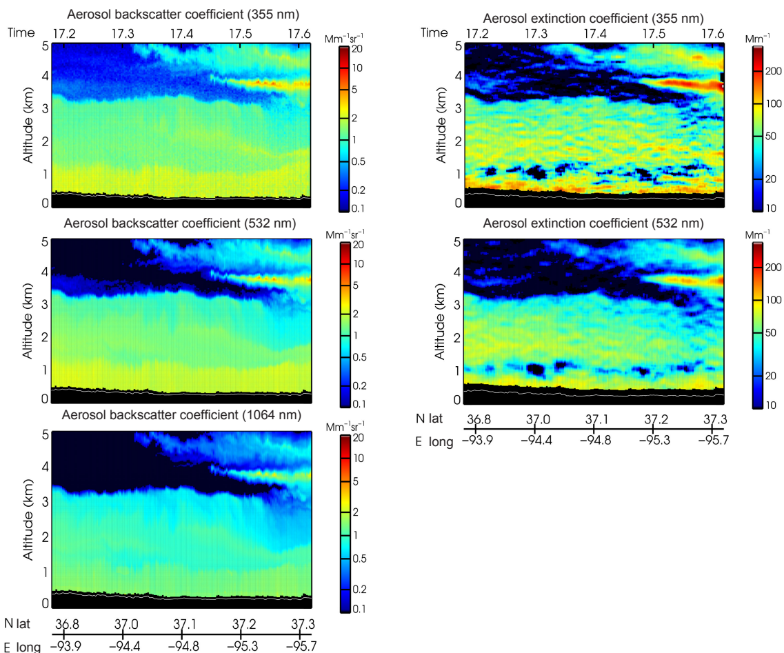
Figure 3. Curtains of aerosol backscatter and extinction coefficients from HSRL-2 for observations on 13 July 2014 for a flight segment in Missouri and Kansas in the midwestern United States.
