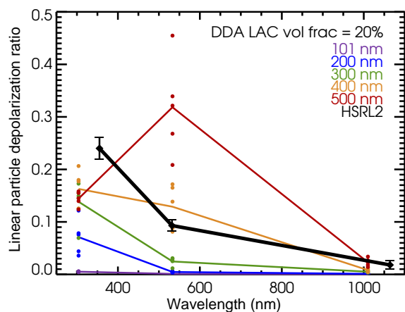
Figure 15. The linear particle depolarization ratio at three wavelengths for soot aggregates embedded in a sulfate shell reproduced from Kahnert et al. (2012), for 20% LAC volume fraction. Dots indicate five realizations with randomly generated geometries, per aggregate volume-equivalent particle radius. The colored lines connect the averages of the five for each wavelength. The legend shows the aggregate volume-equivalent particle radii at which the calculation was performed. The thick black line indicates the particle depolarization ratios measured by airborne HSRL-2 within a smoke plume observed on 17 July 2014 at 355, 532, and 1064 nm.
