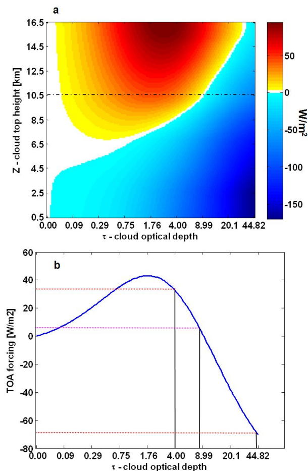
Fig. 4. Upper: \tau - Z space of the cloud radiative forcing at the top of the atmosphere, where \tau denotes the cloud optical depth and Z , the cloud top altitude. The color indicate the top of the atmosphere (TOA) daily average cloud radiation effect in [W/m 2 ] as a function of the cloud height (vertical axis) and cloud optical depth (horizontal axis) for average effective radius ranging from 20 to 40 \mu m in the upper atmosphere and mixed phase starting from -20^\circ to -40^\circ C where full freezing occurs. Warm colors represent a net warming effect, white represents zero net effect and cold colors represent net cooling. Any shift of the clouds to the left and/or up in the \tau - Z space is associated with a shift toward warming. Note how complex the space is, suggesting that averaging of cloud properties ( \tau and Z ) will result in wrong radiative flux estimations. Lower: cross section taken from the above \tau - Z space at Z = 10.5 km, showing top-of-atmosphere (TOA) forcing as a function of cloud optical depth. The bottom figure demonstrates that the mean forcing of anvils with \tau = 4 ( 35 Wm -2 ), covering 90% of the scene, and towers with \tau = 44 ( -68 Wm -2 ), covering 10% of the scene is \sim 25 Wm -2 , is 5 times higher than the forcing calculated for the mean \tau of the scene \tau = 8 , ( 5 Wm -2 ).
