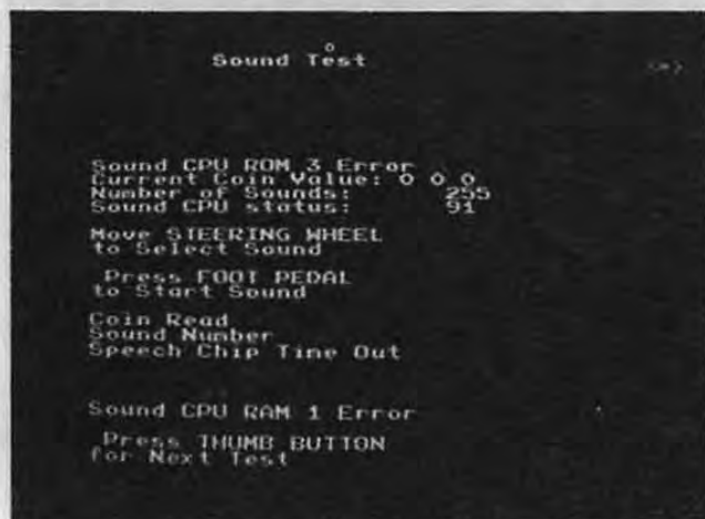
Figure 2-16 Sound Test
