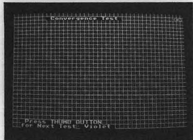
Figure 2-15 Convergence Test
