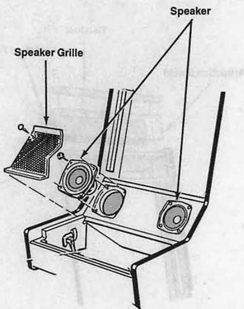
Figure 3-6 Speaker Removal
