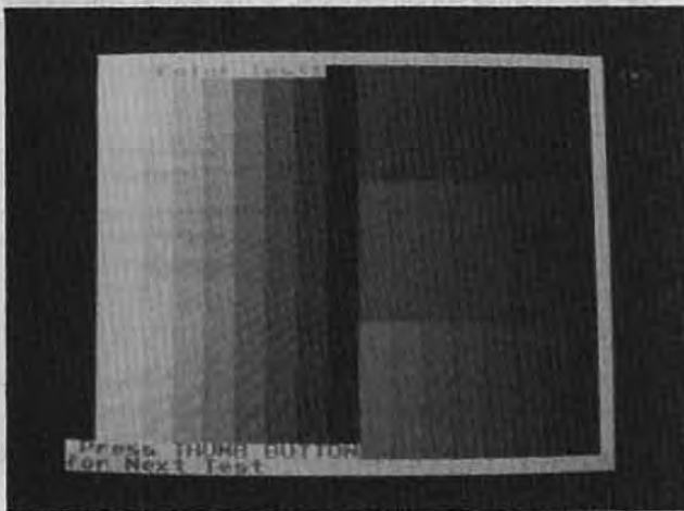
Figure 2-13 Color Test
