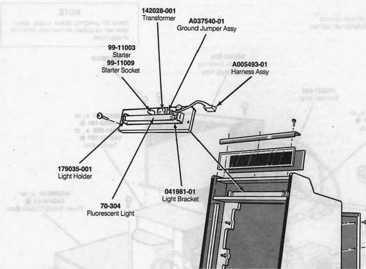
Figure 5-4 Fluorescent Light Panel Assembly A042884-01 A
