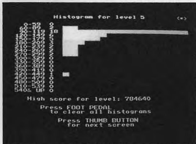
Figure 2-7 Histograms
