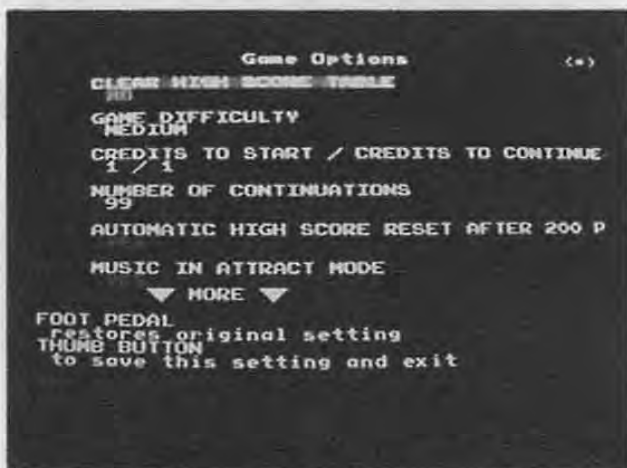
Figure 2-5 Game Options
