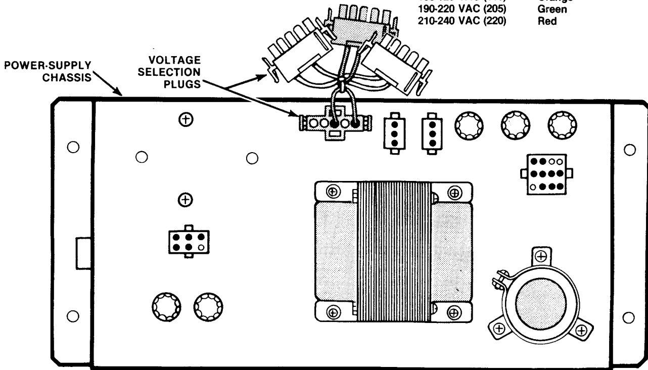
Figure 3 Power Supply
