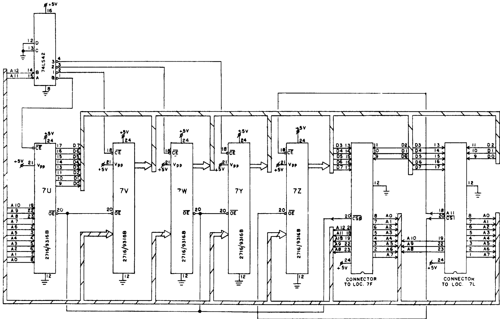
MEMORY LOGIC SCHEMATIC PART NO. M051-00866-A004
