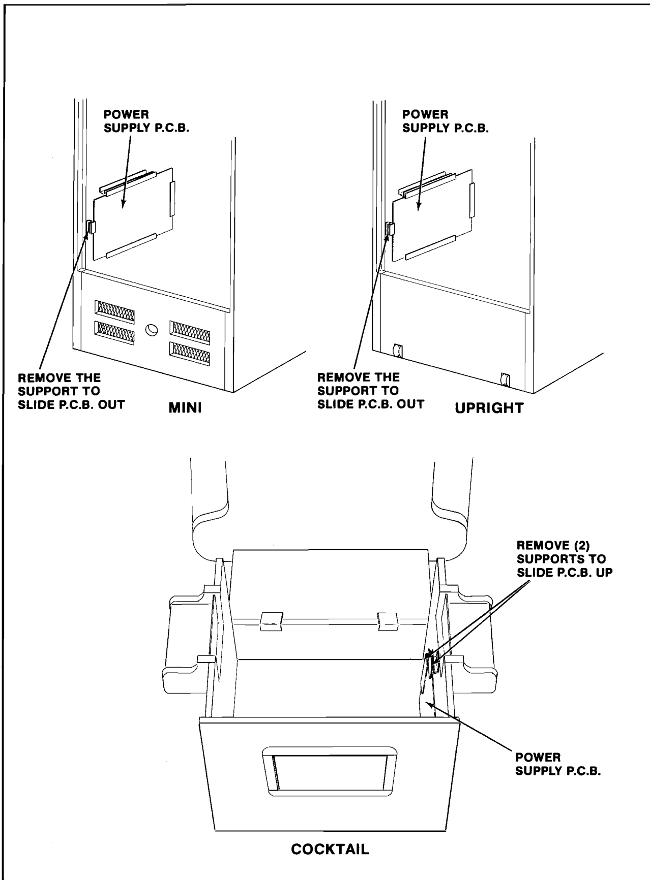
Figure 9. P.C.B. replacement
