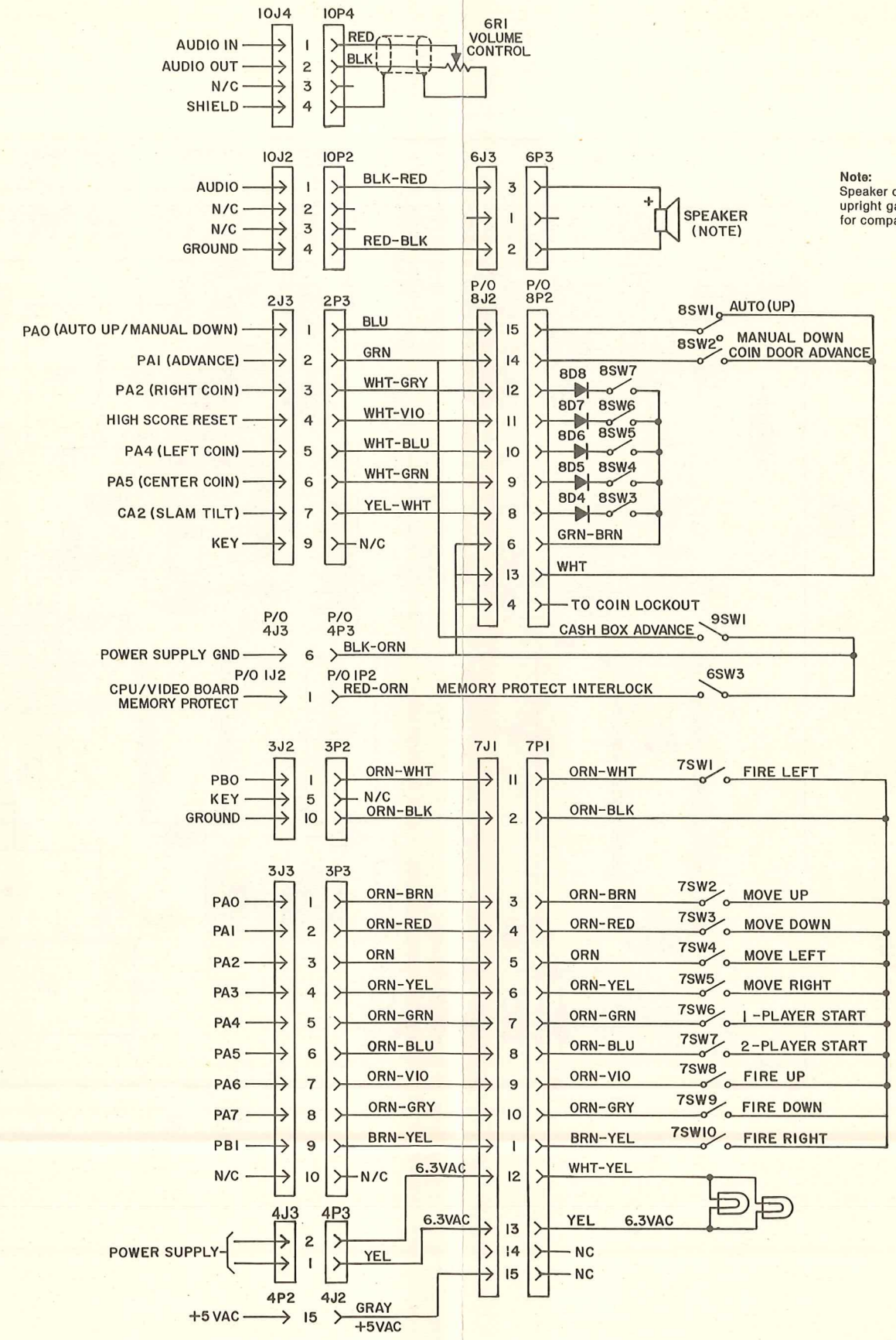
Cabinet Wiring Diagram
