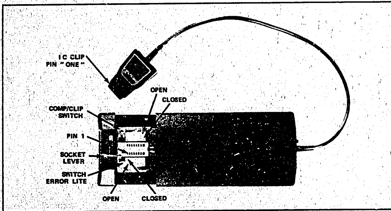
Figure 1. Socket Card
