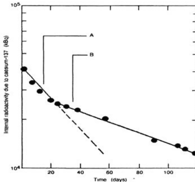
Figure 1. Comparisons of 137 Cs whole body activity during and after Prussian blue insoluble treatment. Line A: 137 Cs whole body activity (kBq) DURING Prussian blue insoluble treatment at 10 gm/day. Line B: 137 Cs whole body activity (kBq) AFTER Prussian blue insoluble treatment is terminated. Dotted line: Extrapolated decrease in 137 Cs whole body activity (kBq) if Prussian blue insoluble treatment was continued.
